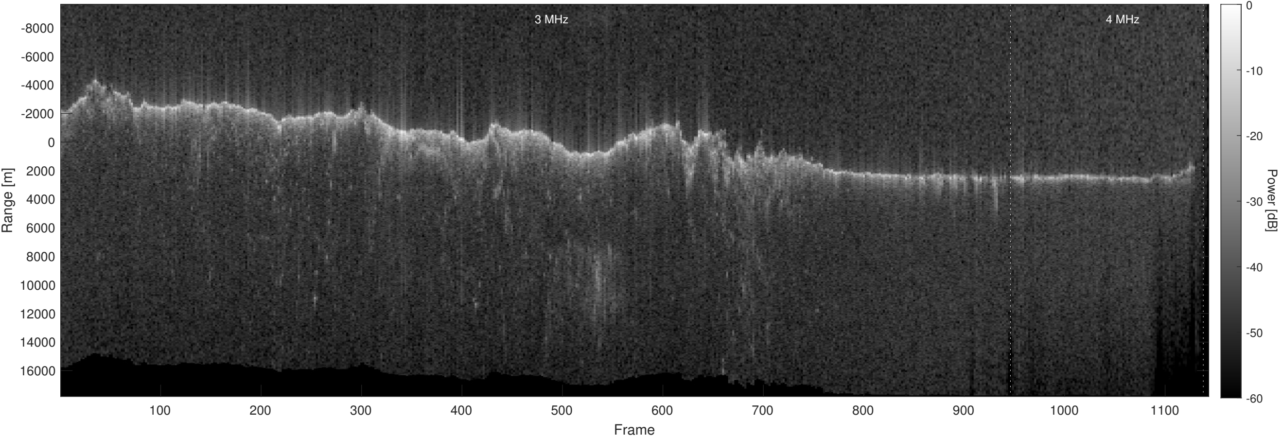
Orbit 10112, Optimized, No Window, Depth-Corrected, Channel 2
