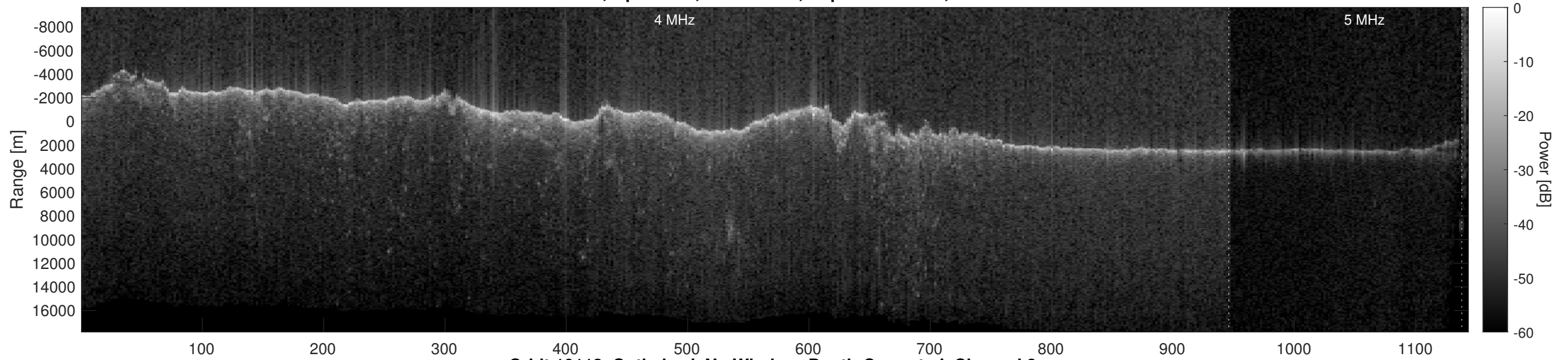
Orbit 10112, Optimized, No Window, Depth-Corrected, Channel 2
