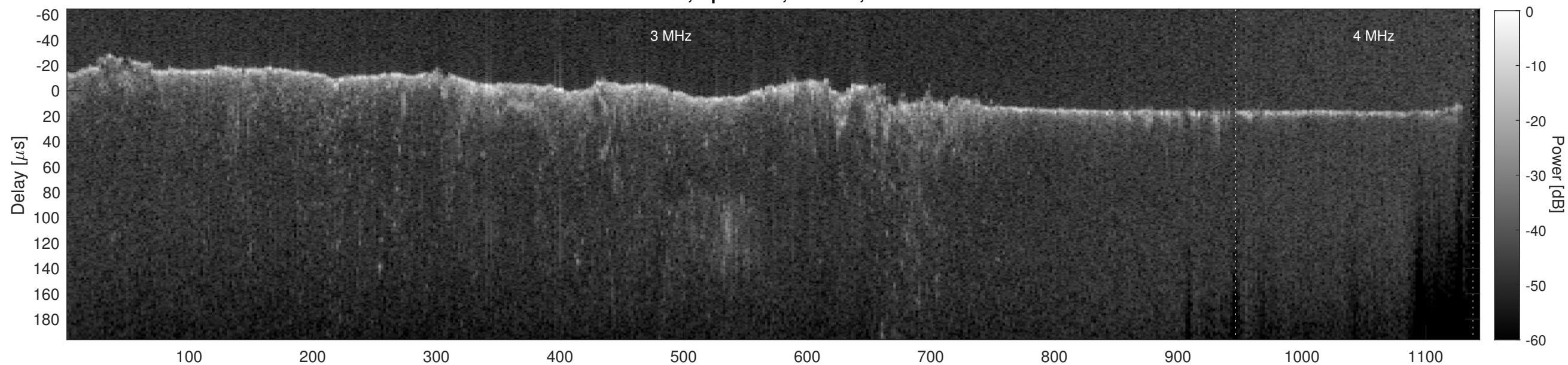
Orbit 10112, Cluttergram
