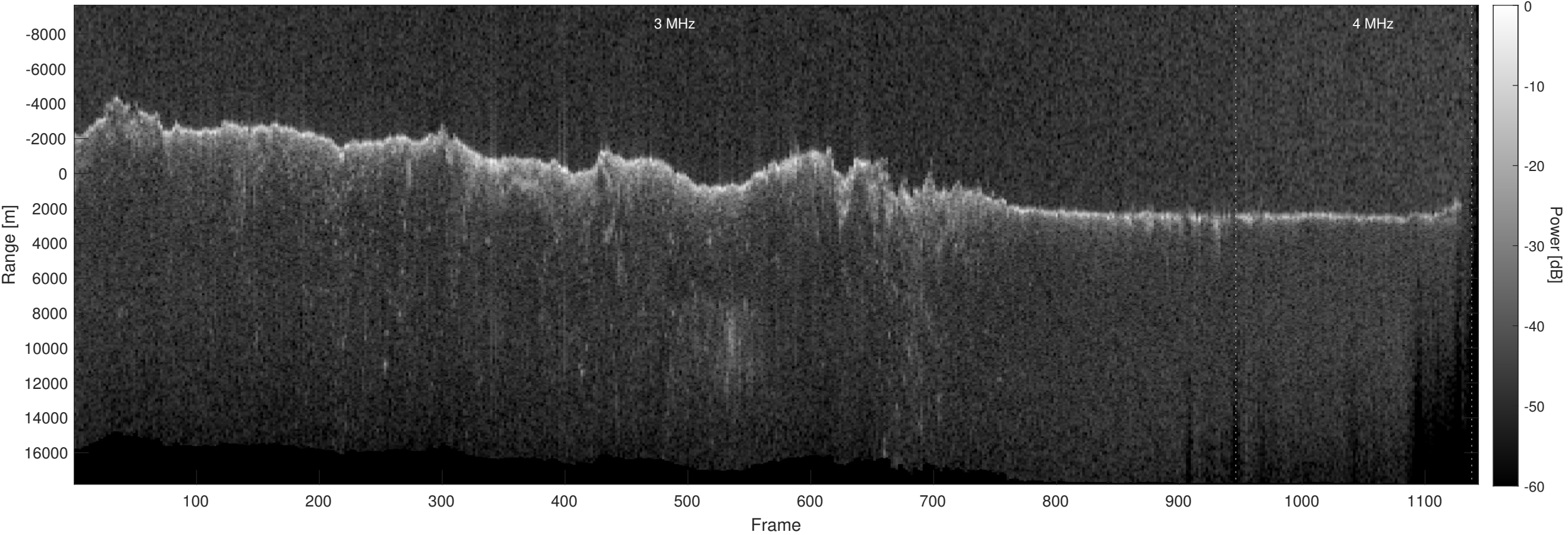
Orbit 10112, Optimized, Window, Depth-Corrected, Channel 2
