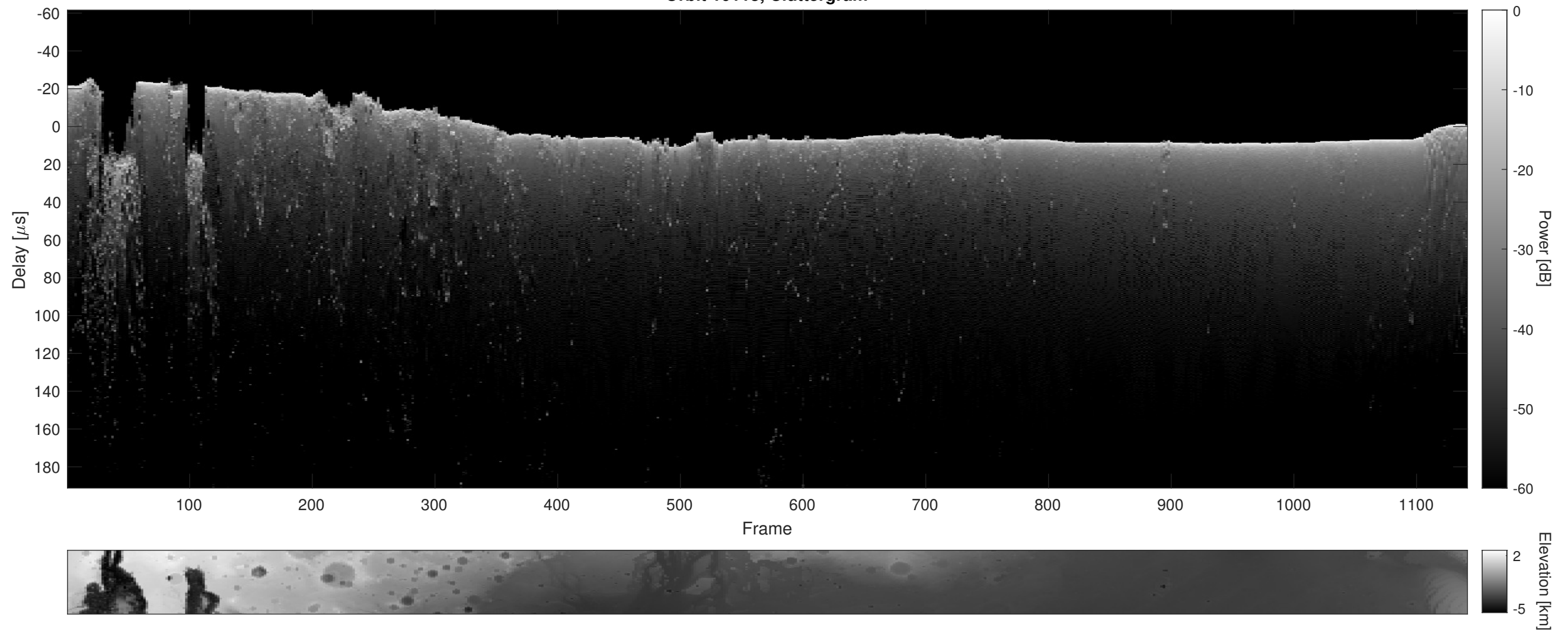
Orbit 10113, Cluttergram
