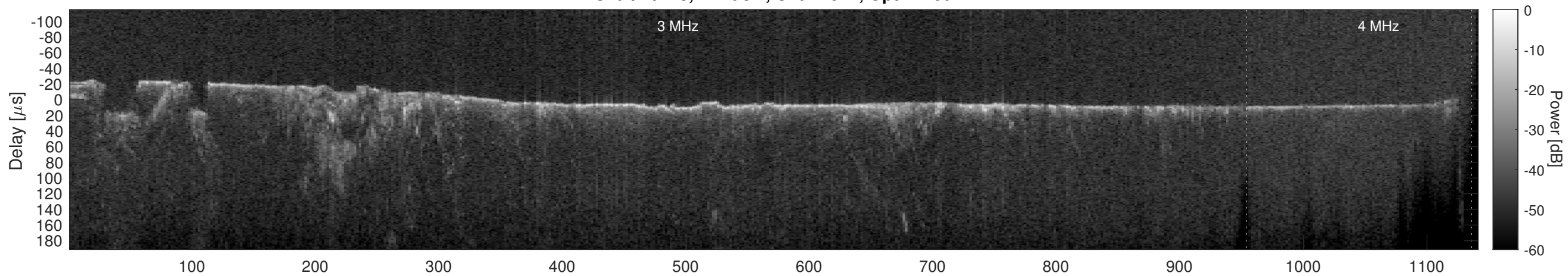
Orbit 10113, Cluttergram
