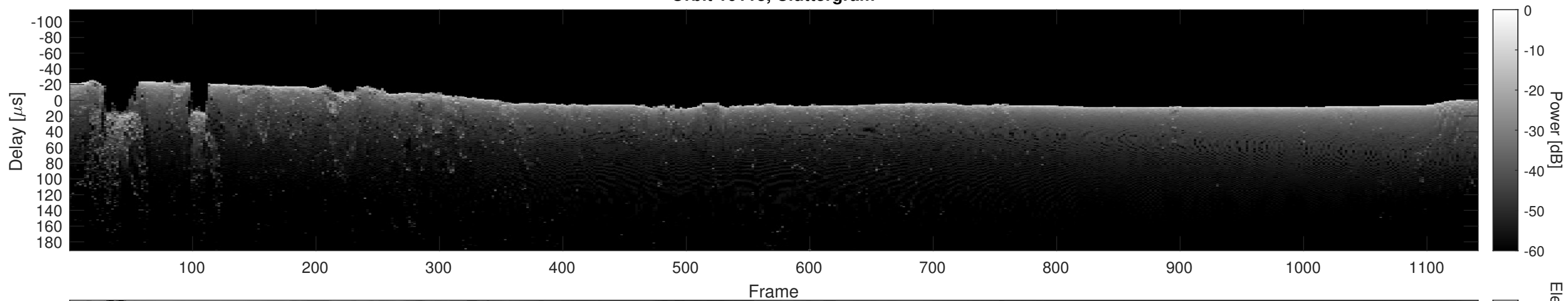
Orbit 10113, Cluttergram
