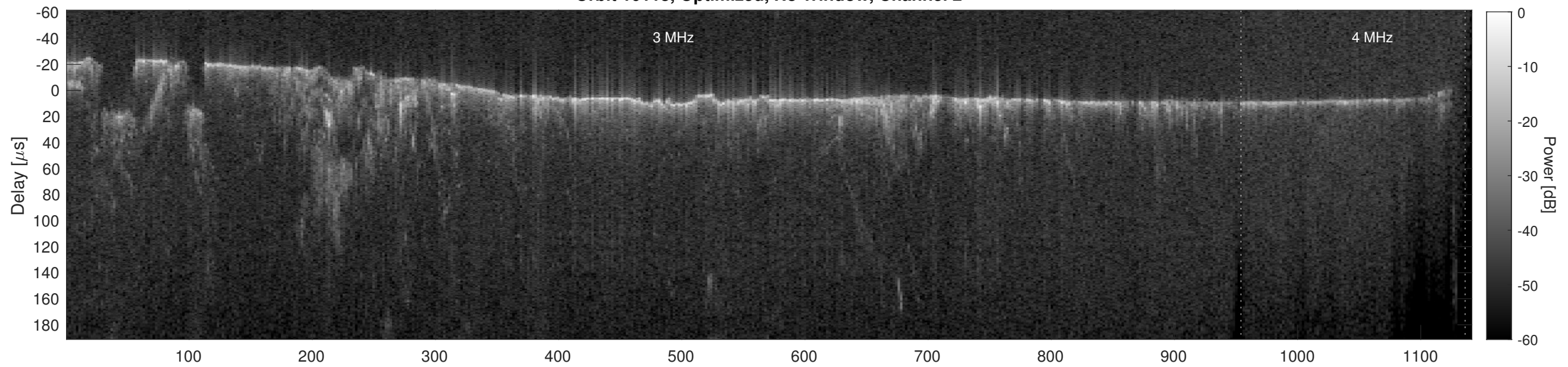
Orbit 10113, Cluttergram
