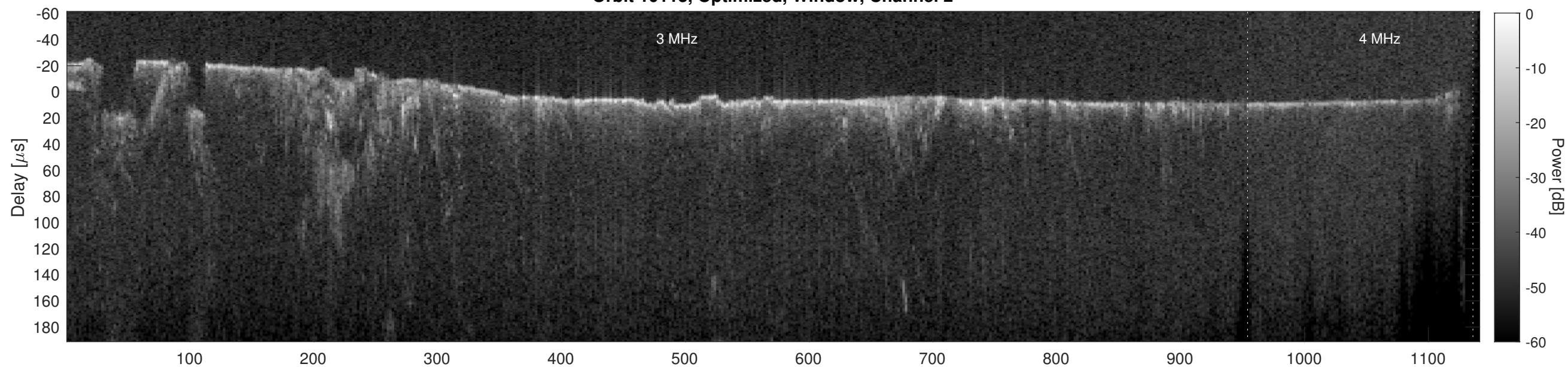
Orbit 10113, Cluttergram
