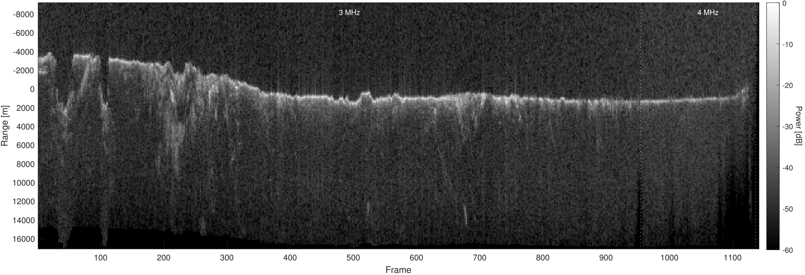
Orbit 10113, Optimized, Window, Depth-Corrected, Channel 2
