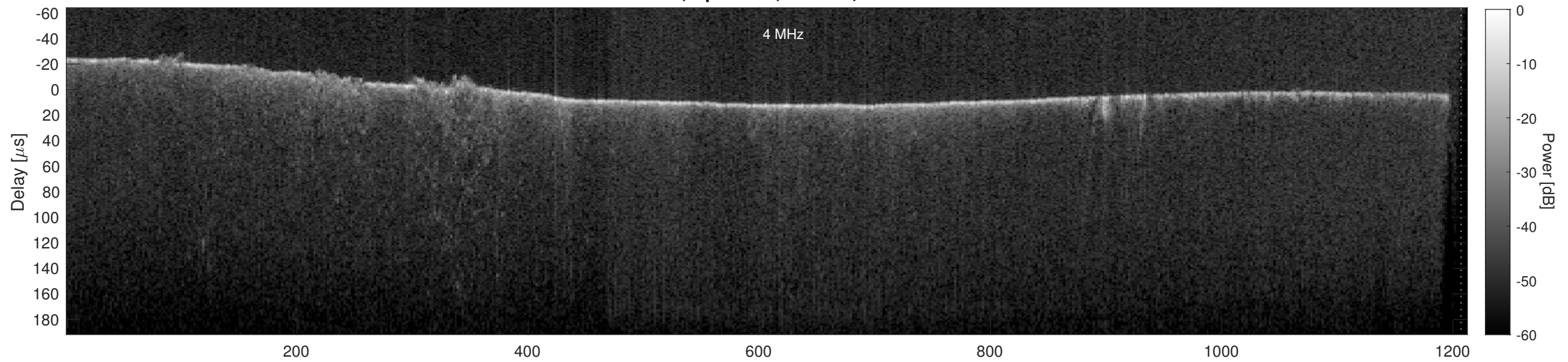
Orbit 10115, Cluttergram
