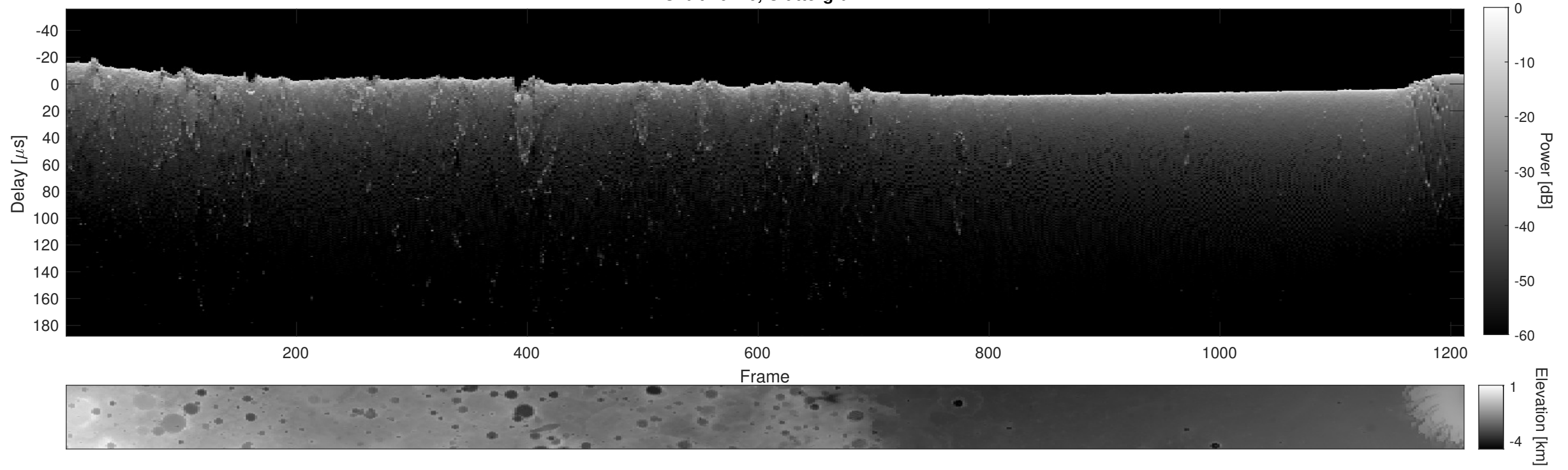
Orbit 10116, Cluttergram
