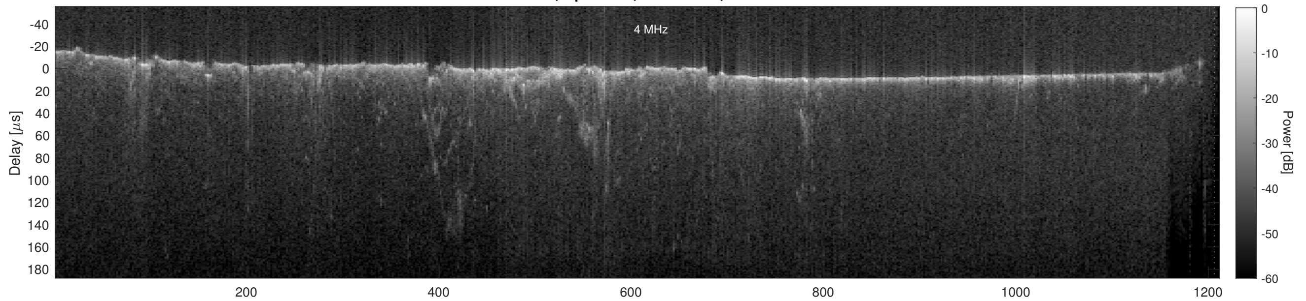
Orbit 10116, Cluttergram
