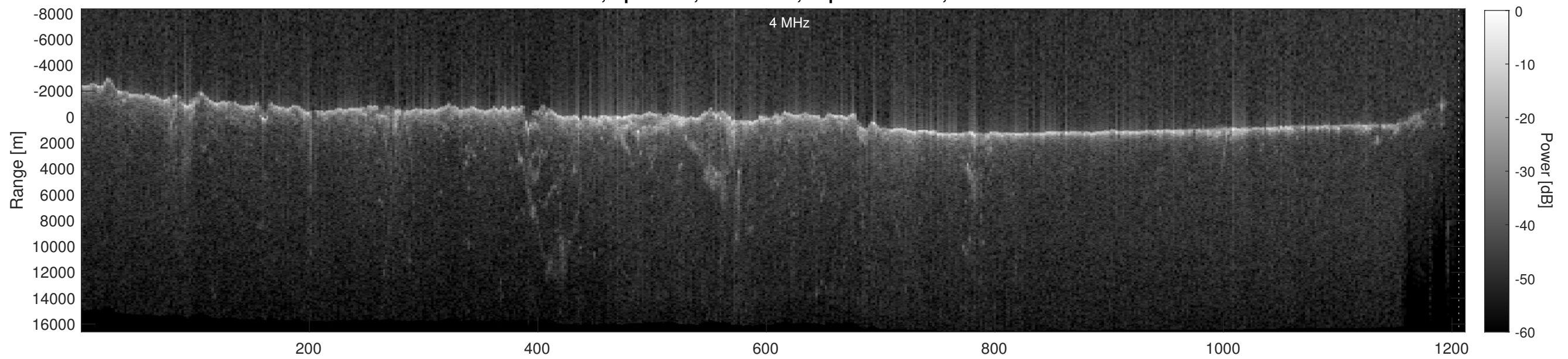
Orbit 10116, Depth-Corrected Cluttergram
