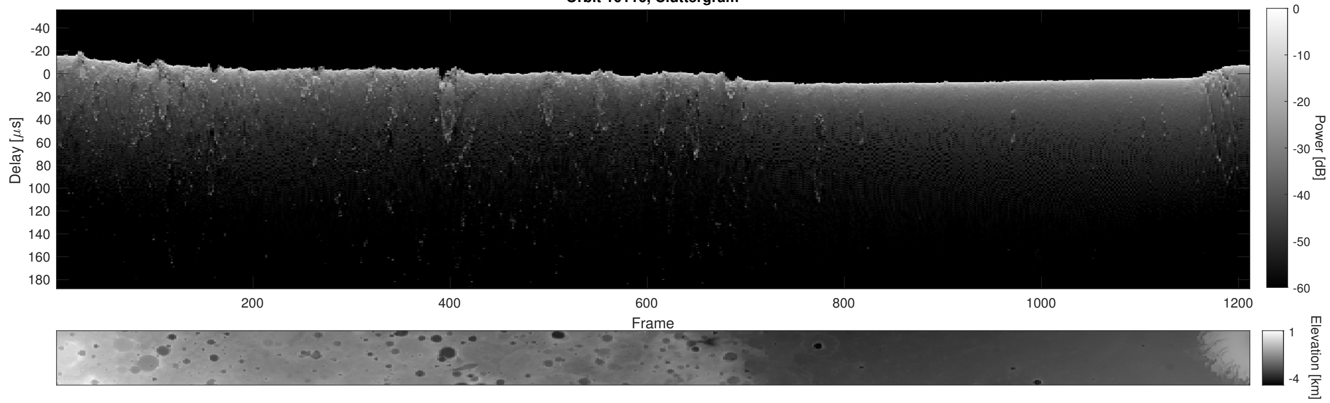
Orbit 10116, Cluttergram
