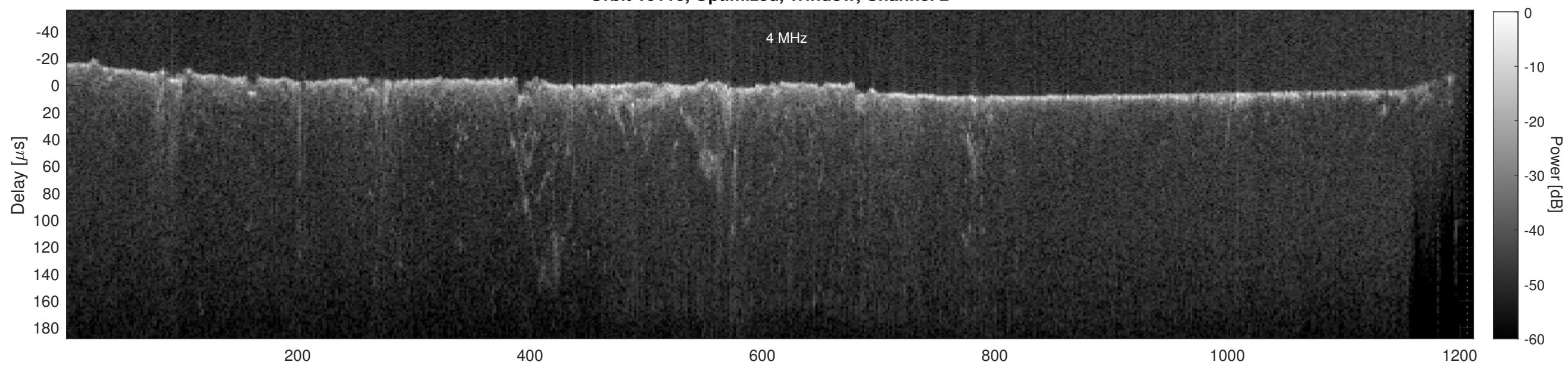
Orbit 10116, Cluttergram
