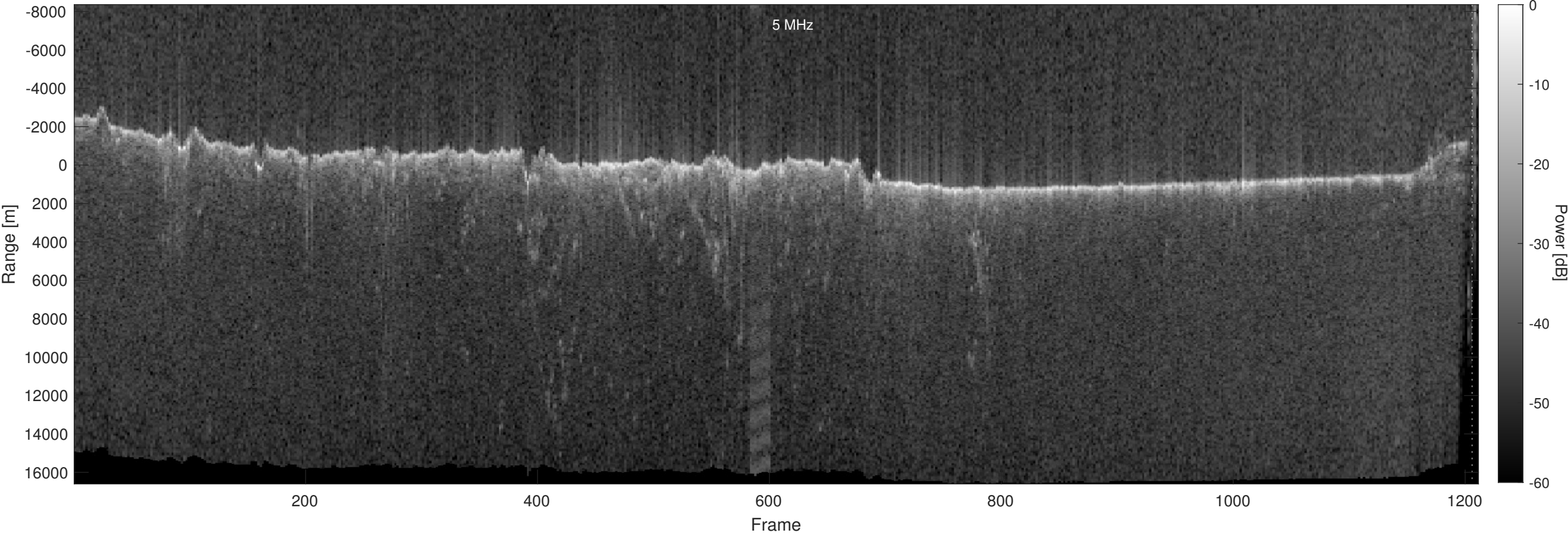
Orbit 10116, Optimized, Window, Depth-Corrected, Channel 2
