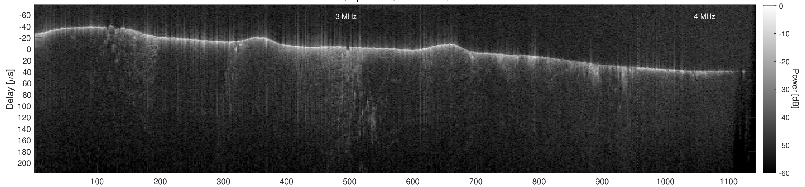
Orbit 10117, Cluttergram
