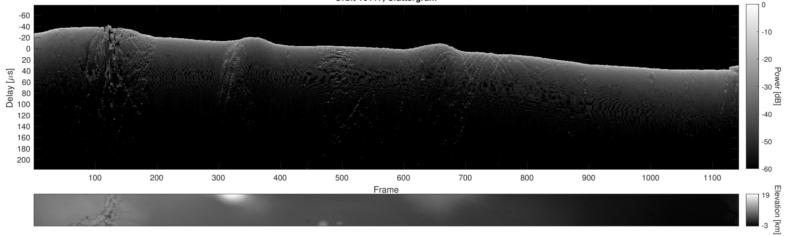
Orbit 10117, Cluttergram
