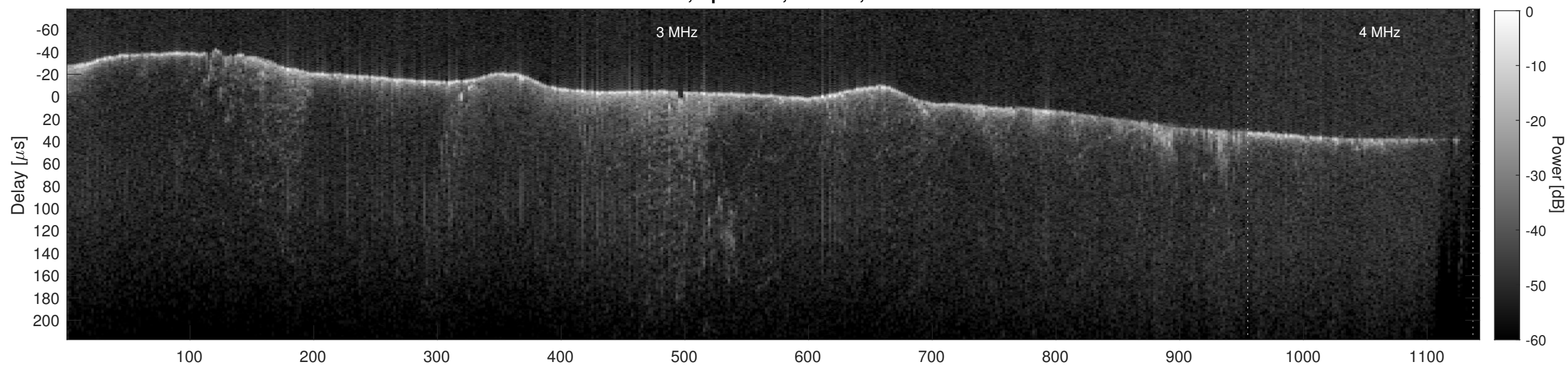
Orbit 10117, Cluttergram
