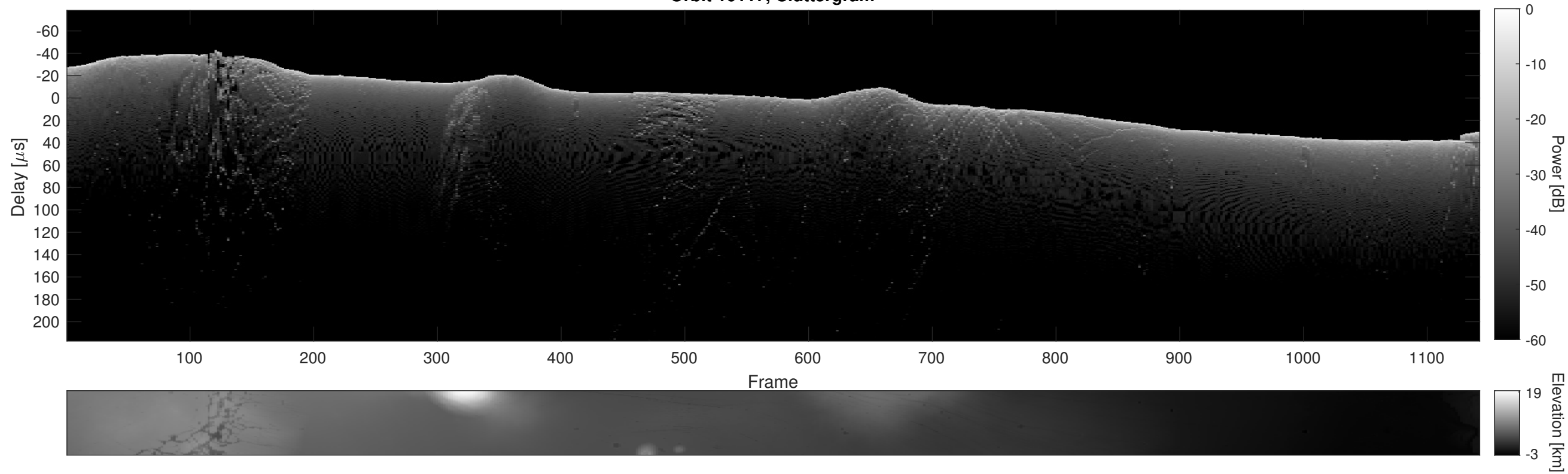
Orbit 10117, Cluttergram
