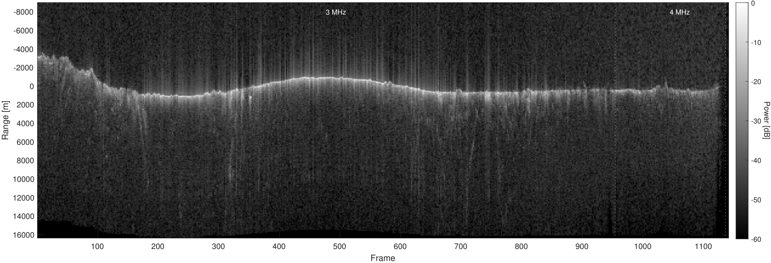
Orbit 10118, Optimized, No Window, Depth-Corrected, Channel 2
