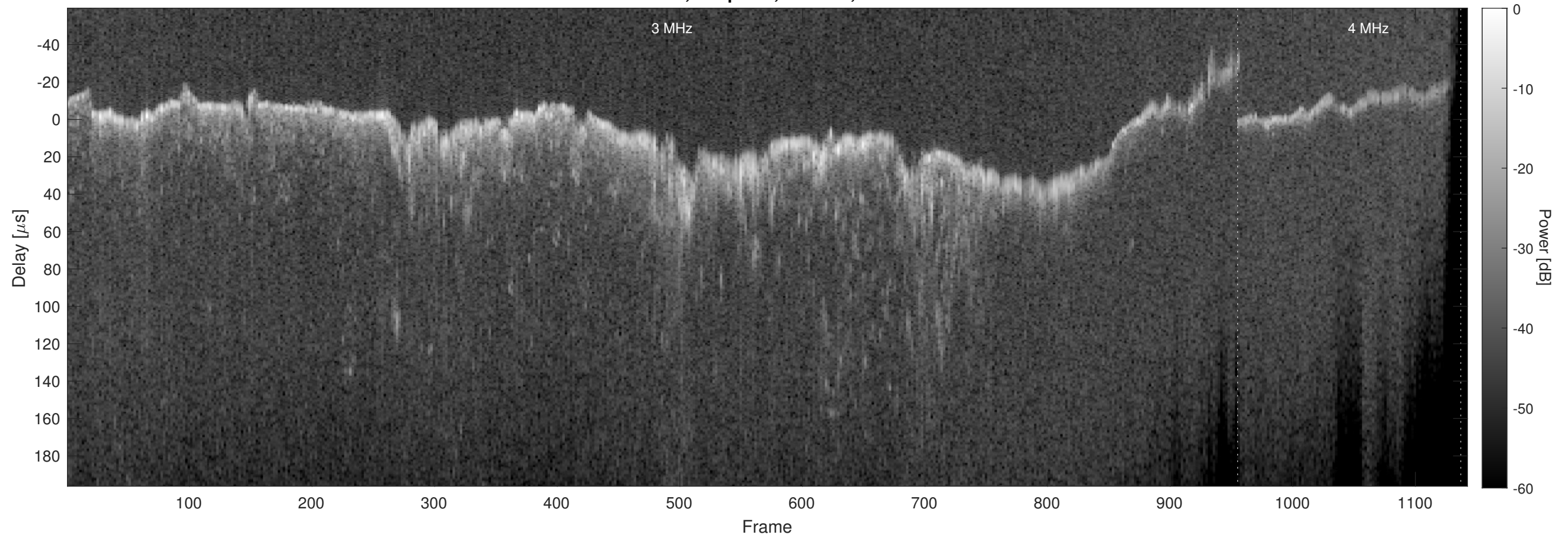
Orbit 10119, Chapman, Window, Channel 2
