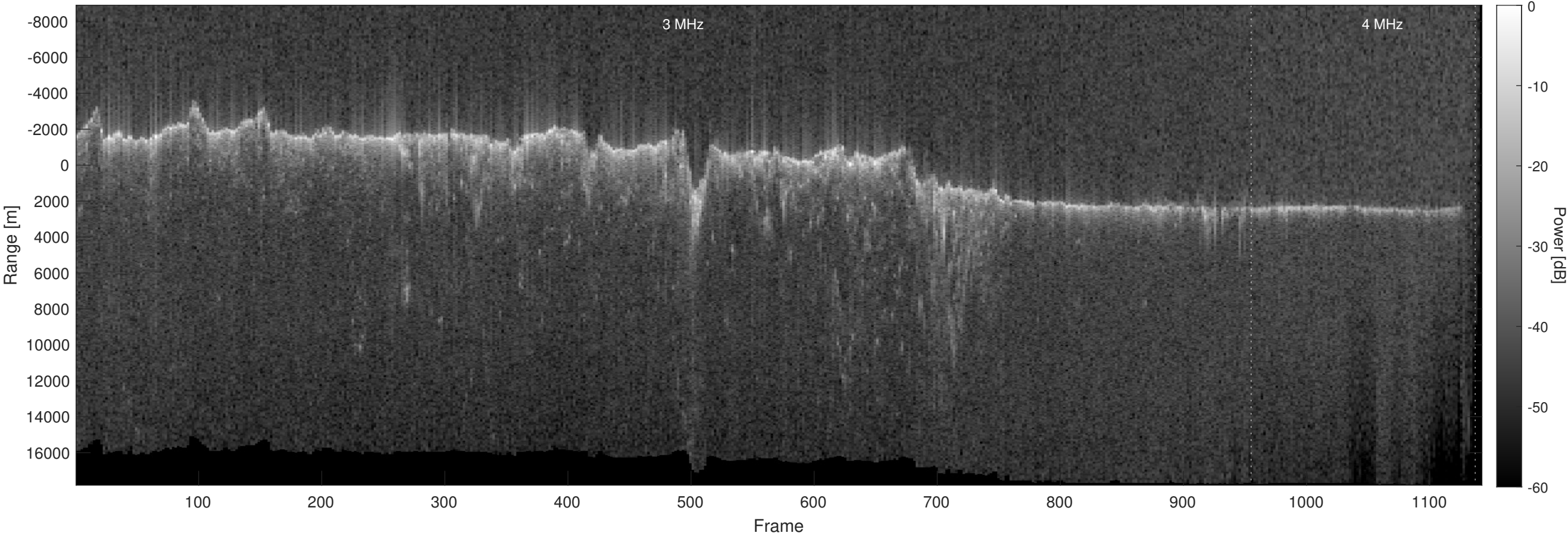
Orbit 10119, Optimized, No Window, Depth-Corrected, Channel 2
