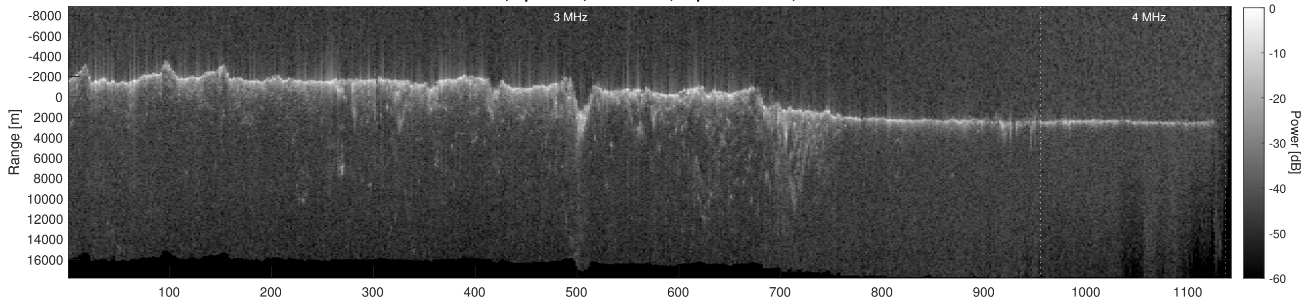
Orbit 10119, Depth-Corrected Cluttergram
