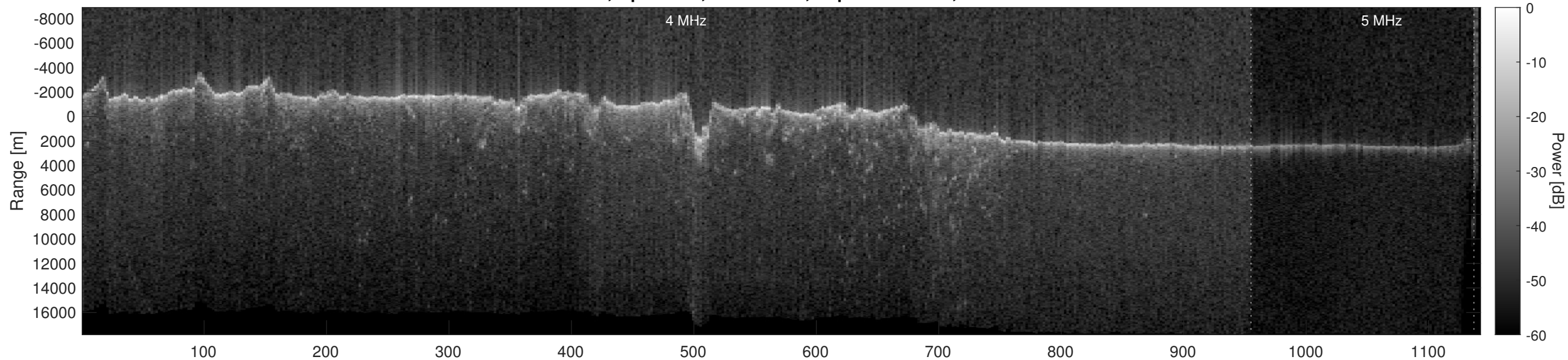
Orbit 10119, Optimized, No Window, Depth-Corrected, Channel 2
