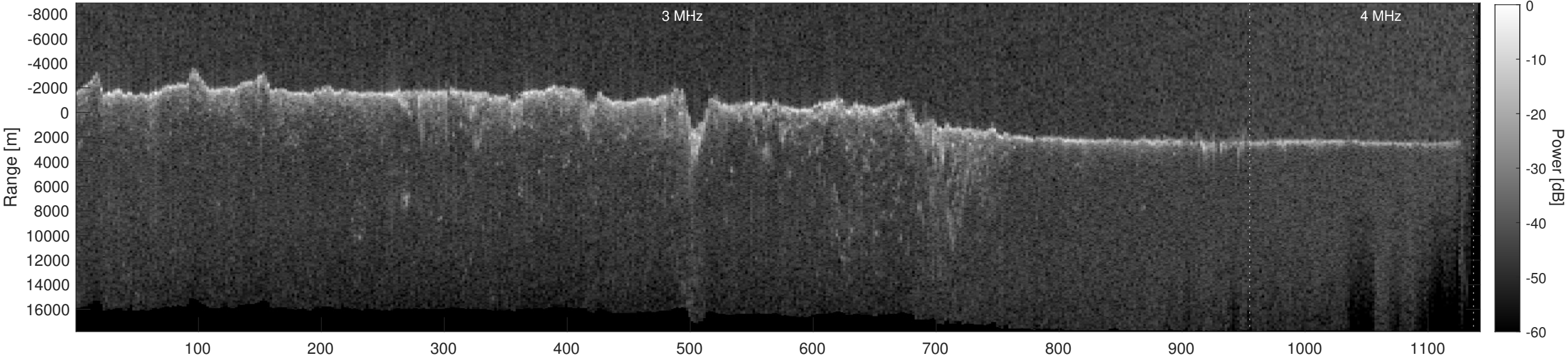
Orbit 10119, Depth-Corrected Cluttergram
