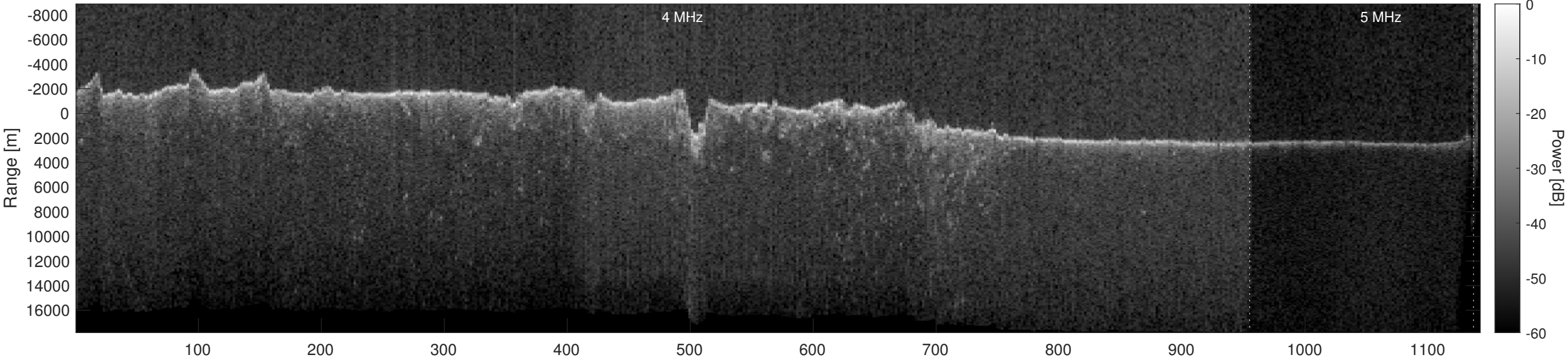
Orbit 10119, Optimized, Window, Depth-Corrected, Channel 2
