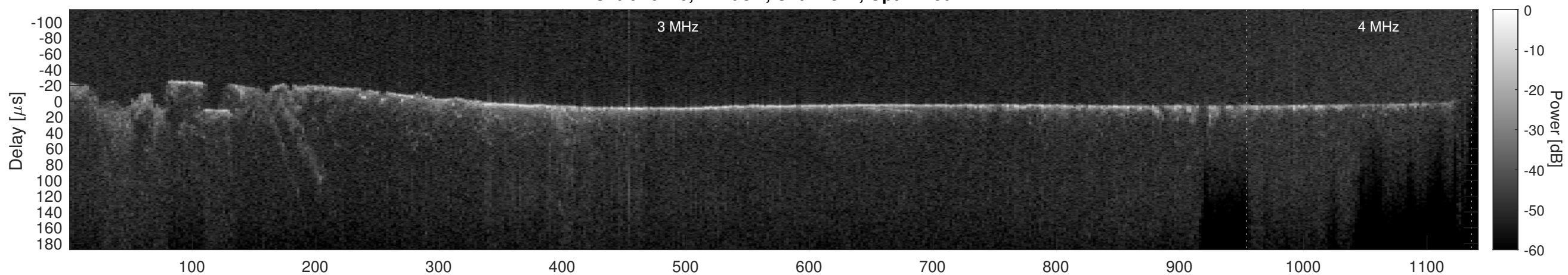
Orbit 10120, Cluttergram
