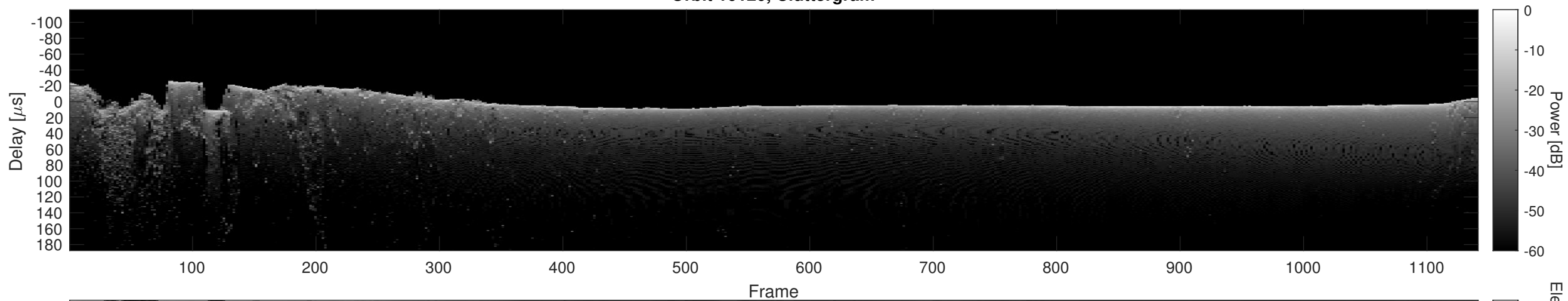
Orbit 10120, Cluttergram
