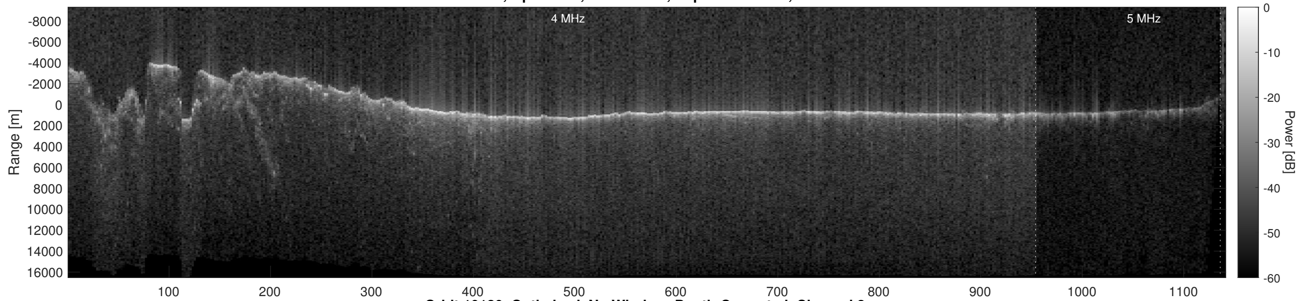
Orbit 10120, Optimized, No Window, Depth-Corrected, Channel 2
