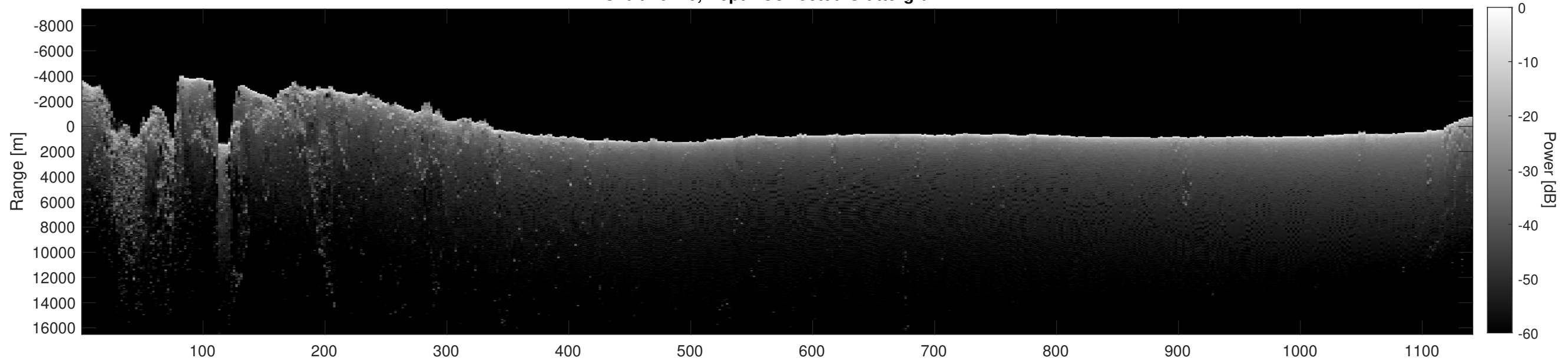
Orbit 10120, Depth-Corrected Cluttergram
