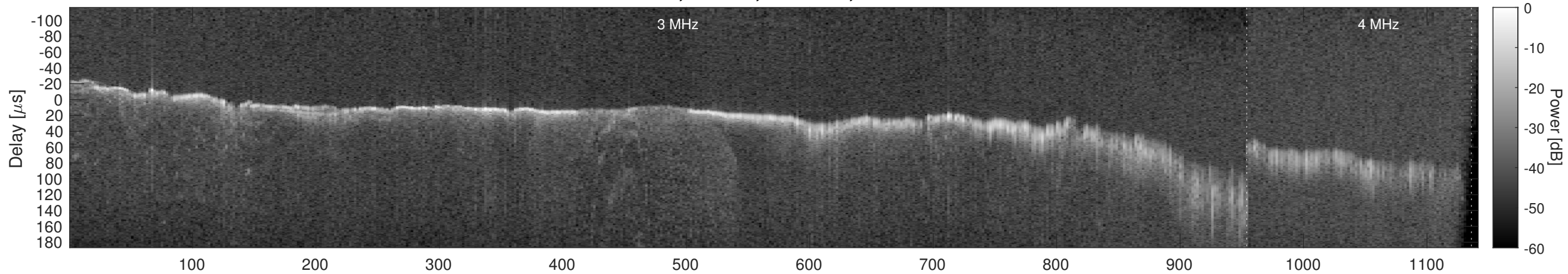
Orbit 10121, Window, Channel 2, Chapman
