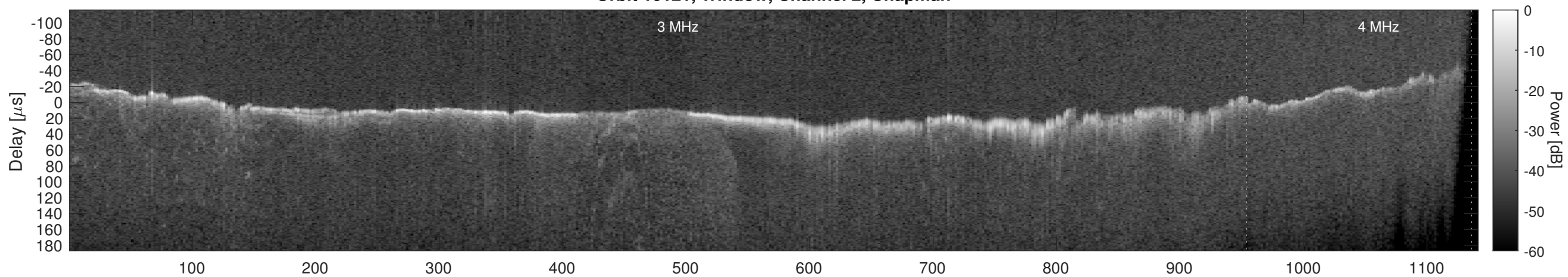
Orbit 10121, Window, Channel 2, Optimized
