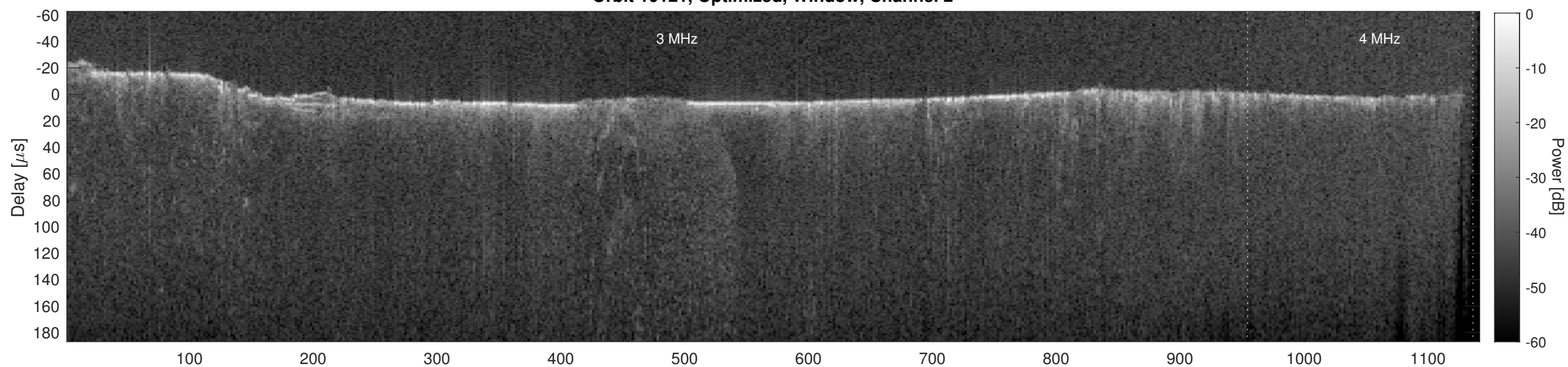
Orbit 10121, Cluttergram
