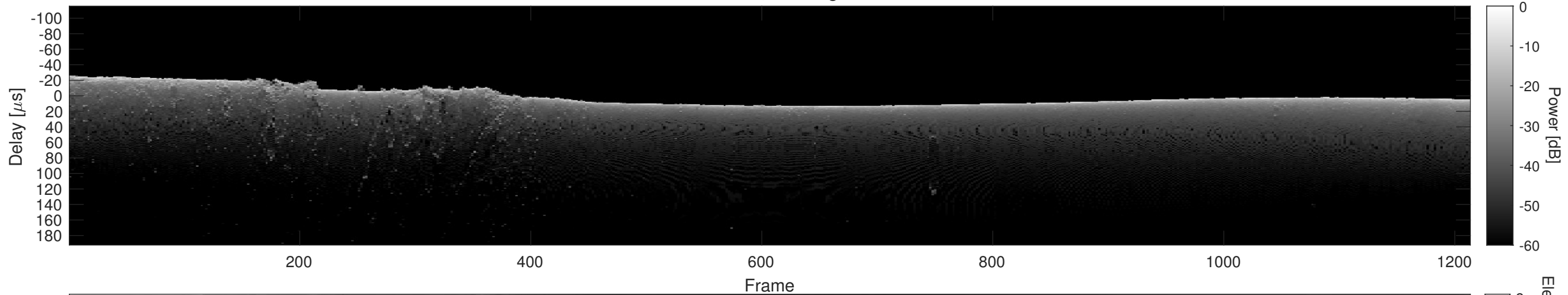
Orbit 10122, Cluttergram
