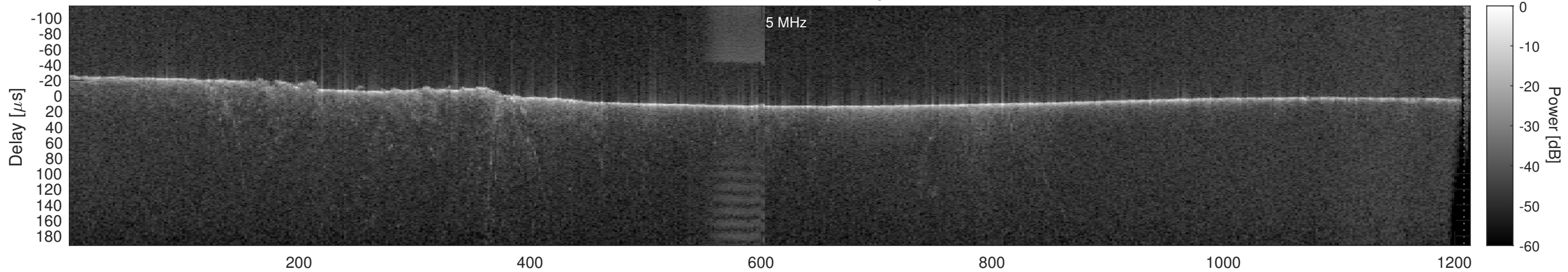
Orbit 10122, Cluttergram
