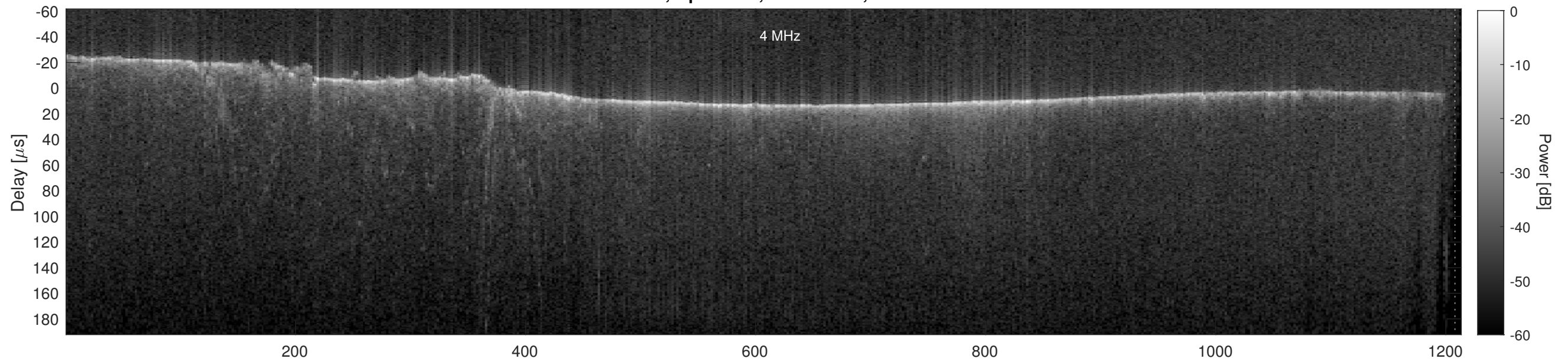
Orbit 10122, Cluttergram
