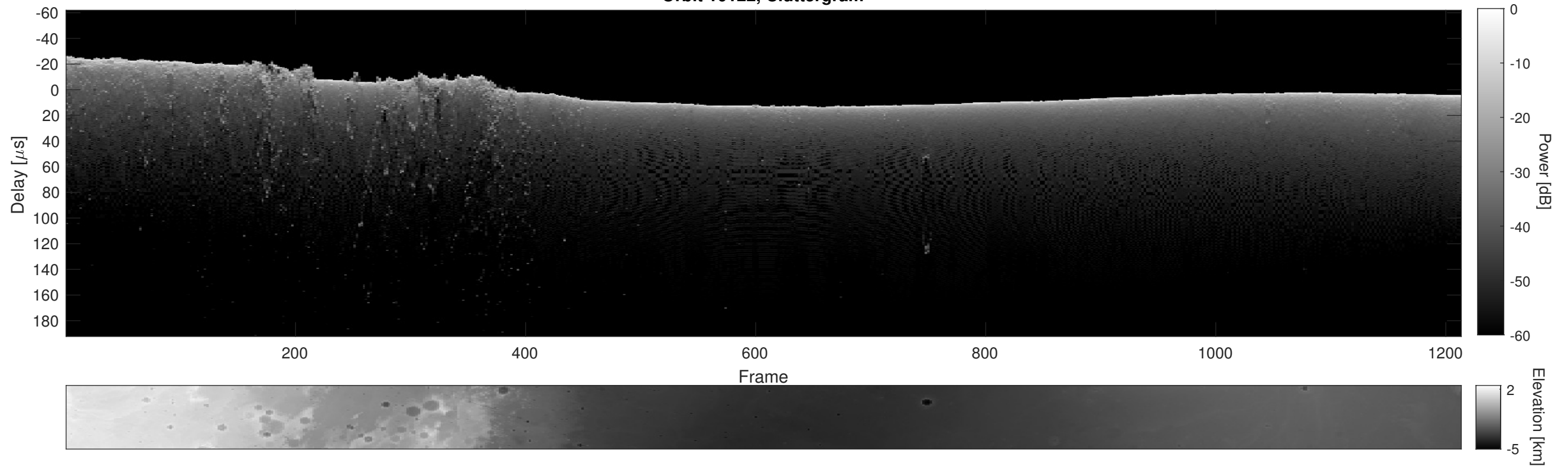
Orbit 10122, Cluttergram
