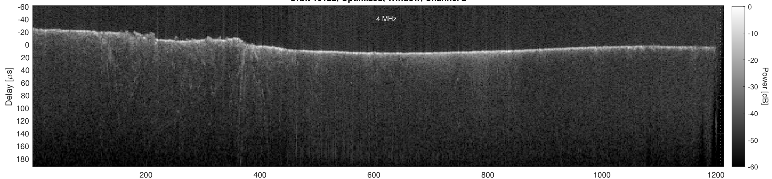
Orbit 10122, Cluttergram
