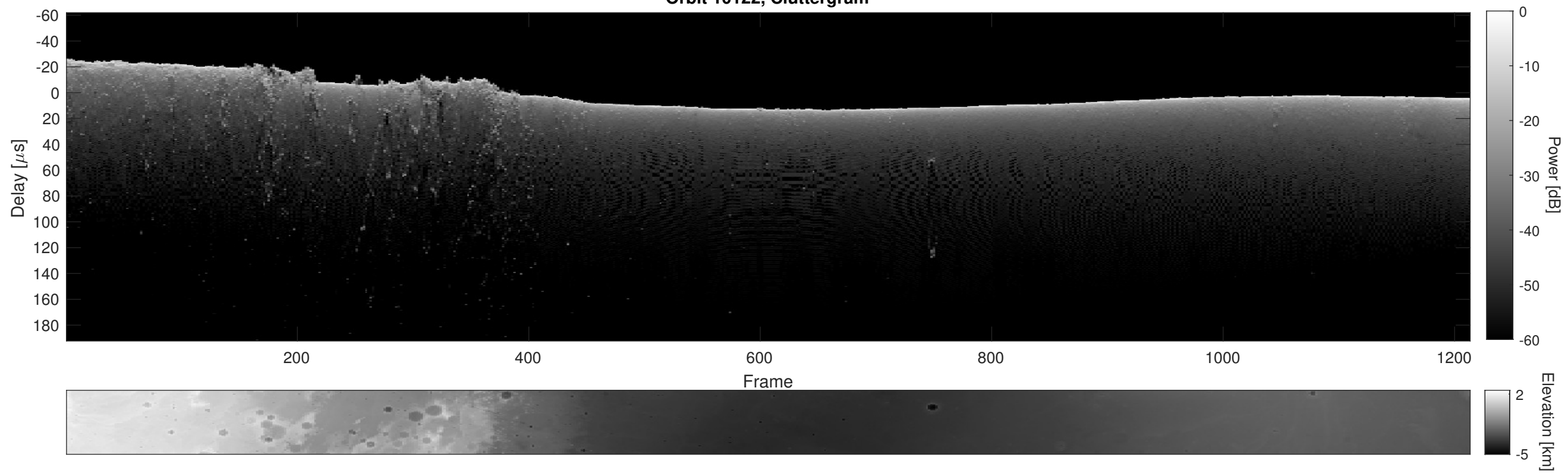
Orbit 10122, Cluttergram
