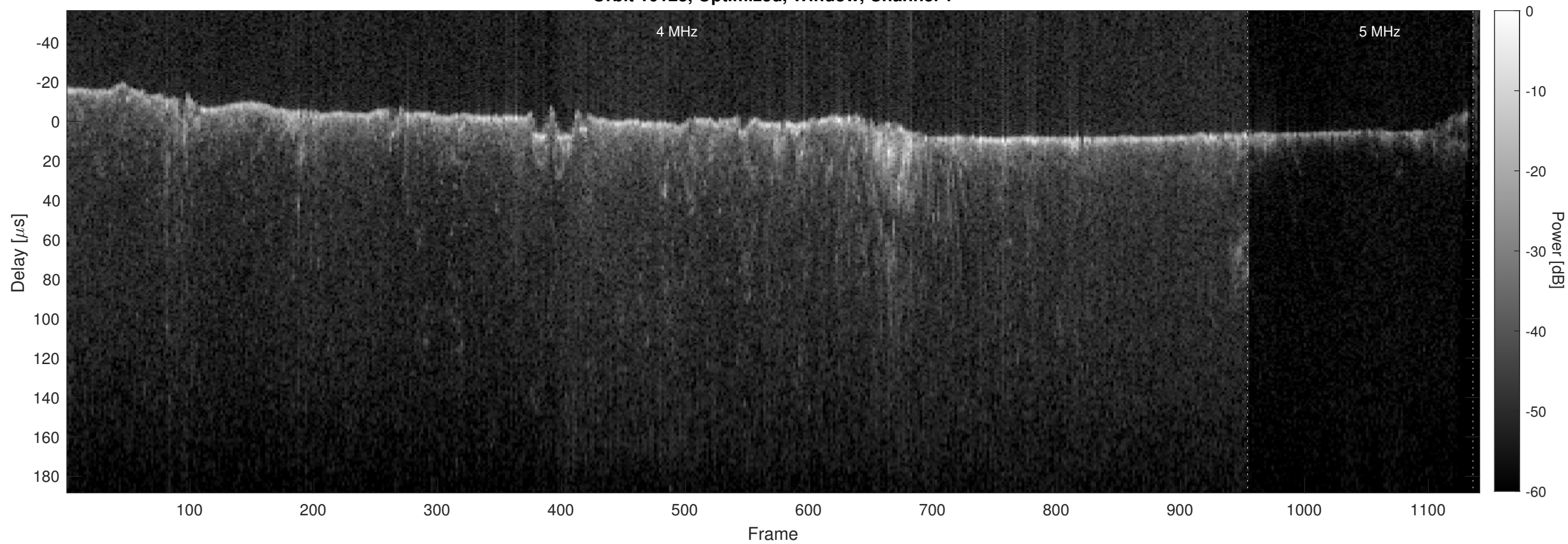
Orbit 10123, Optimized, Window, Channel 2
