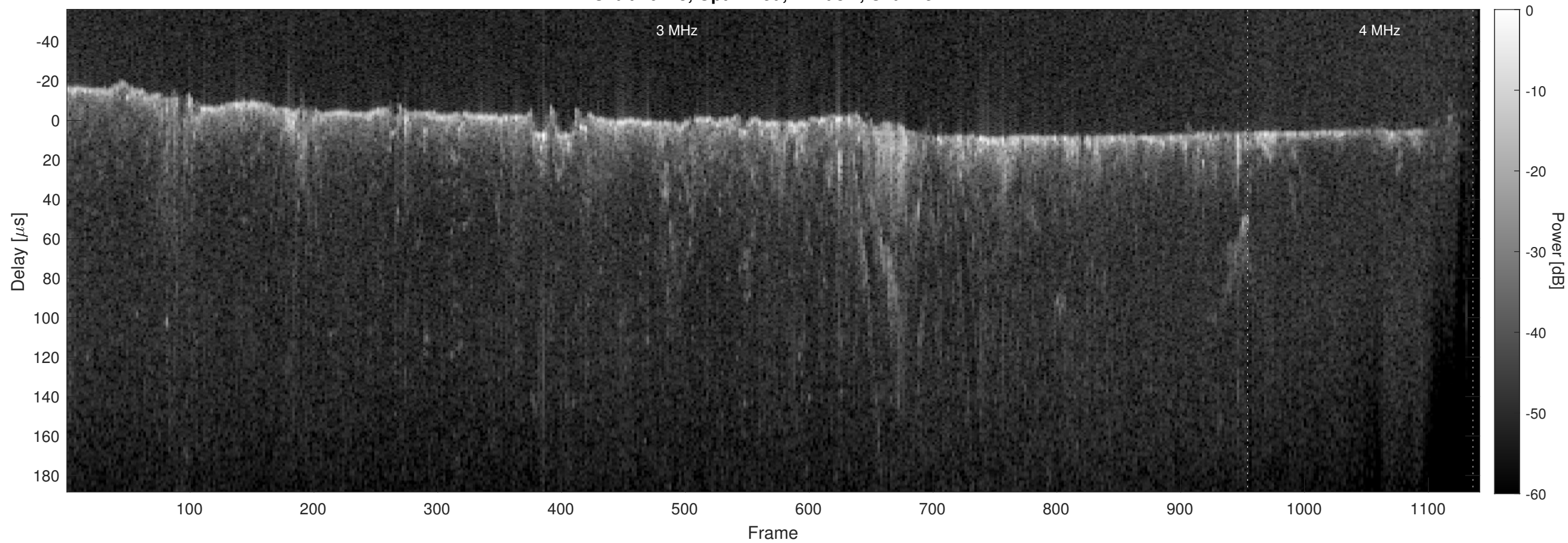
Orbit 10123, Optimized, Window, Channel 2
