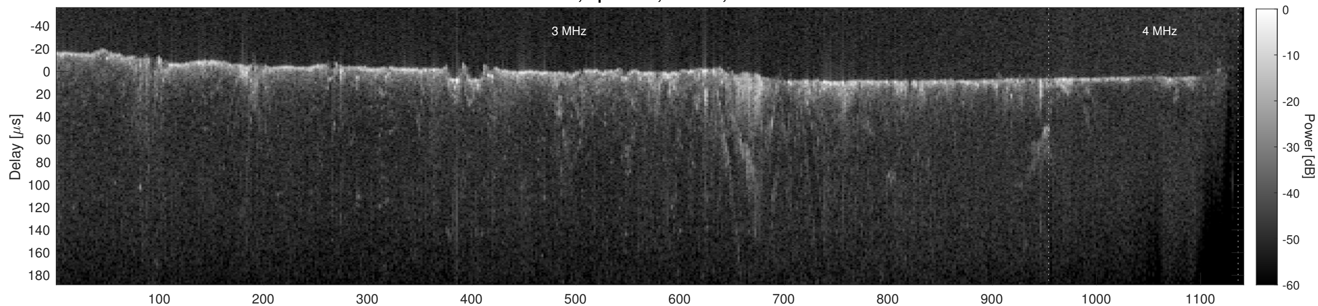
Orbit 10123, Cluttergram
