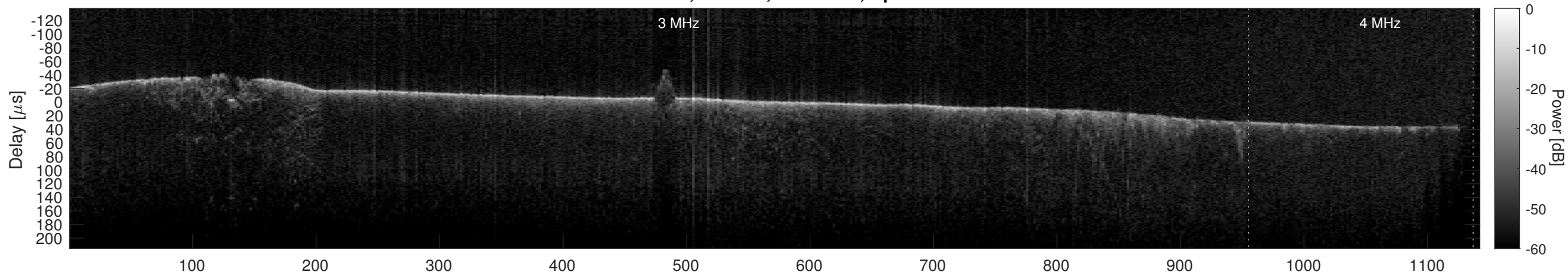
Orbit 10124, Cluttergram
