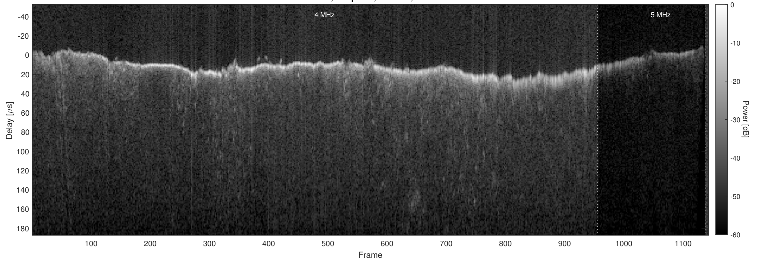
Orbit 10125, Chapman, Window, Channel 2
