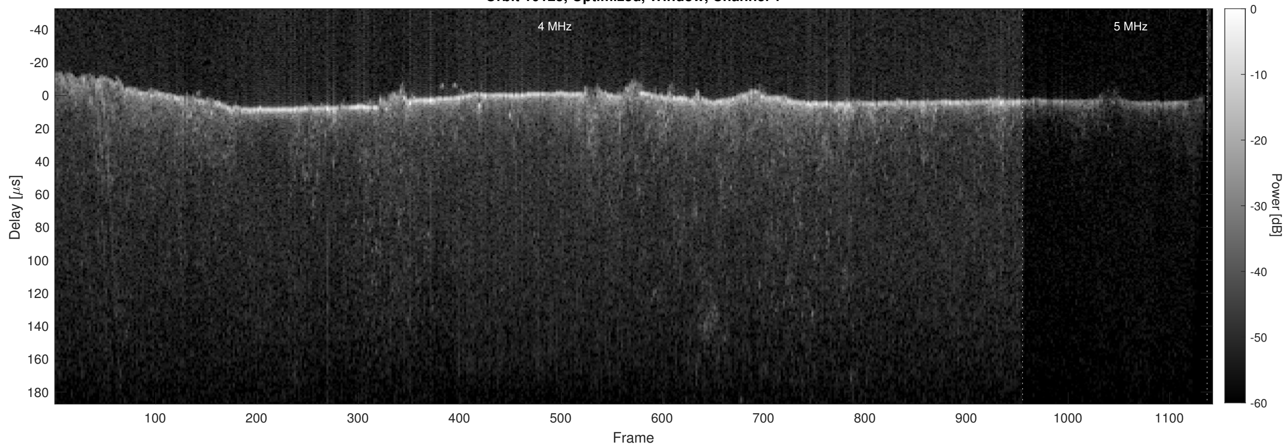
Orbit 10125, Optimized, Window, Channel 2
