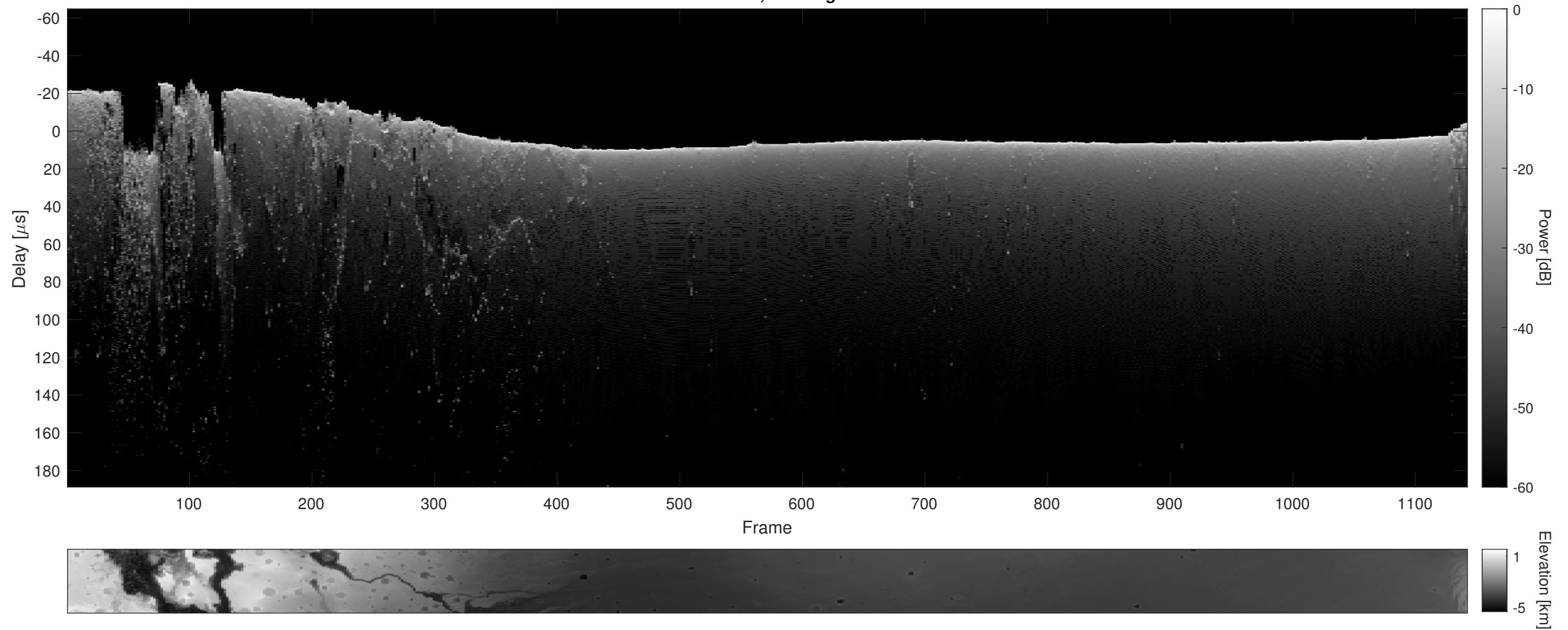
Orbit 10127, Cluttergram
