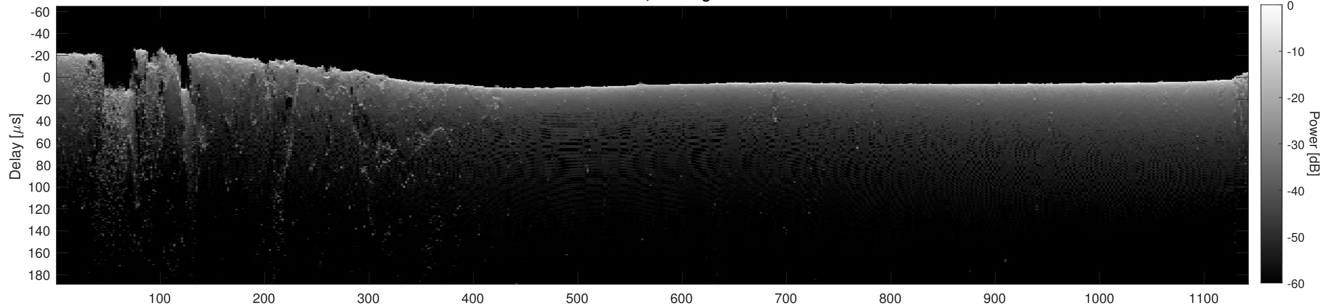
Orbit 10127, Cluttergram
