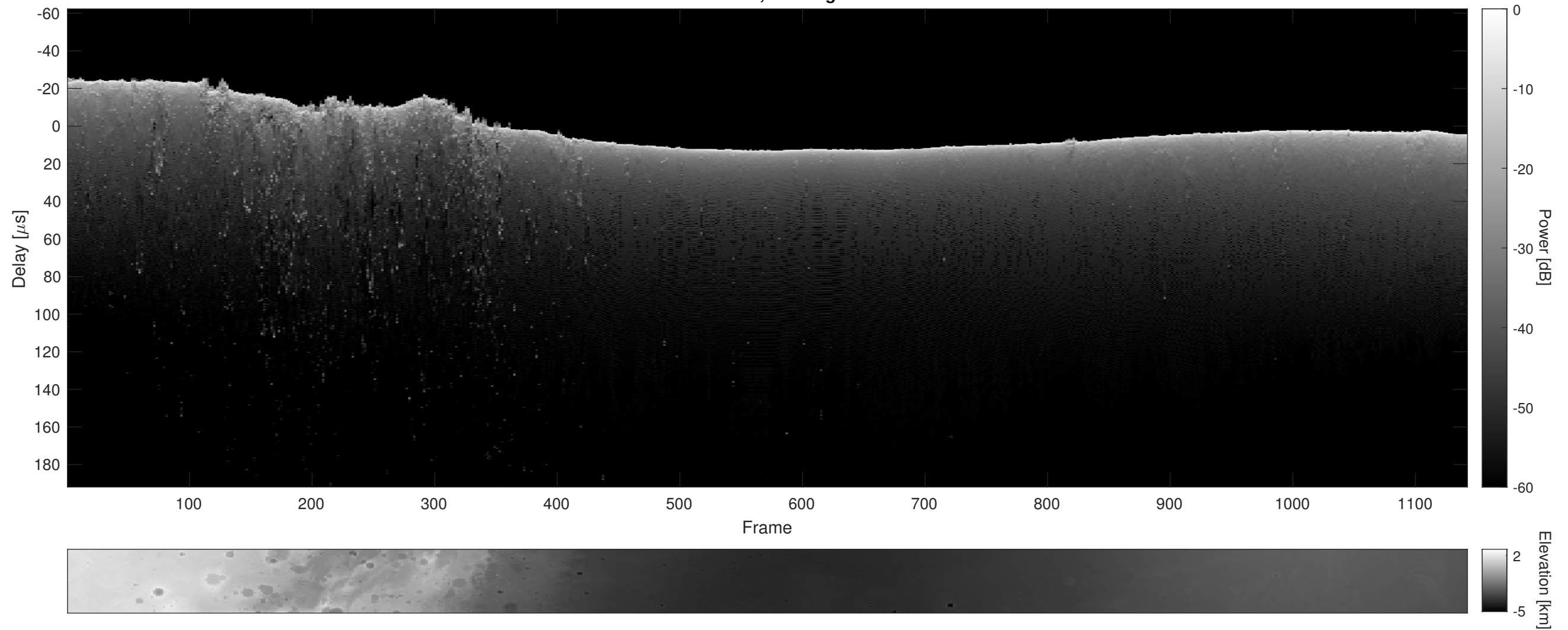
Orbit 10129, Cluttergram
