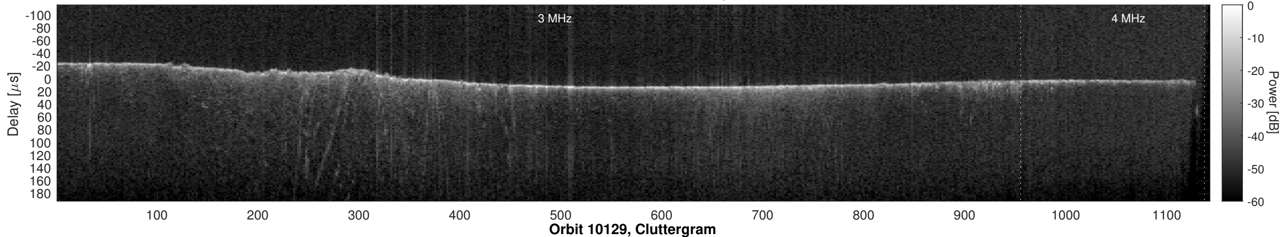
Orbit 10129, Window, Channel 2, Optimized
