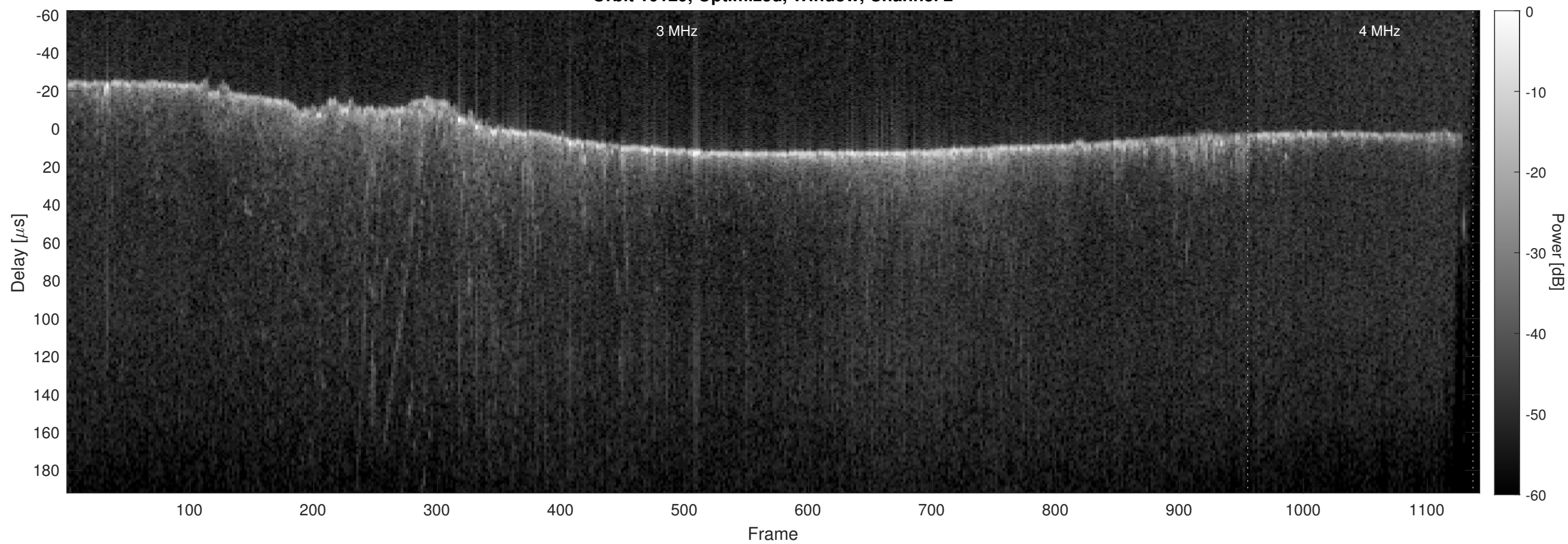
Orbit 10129, Optimized, Window, Channel 2
