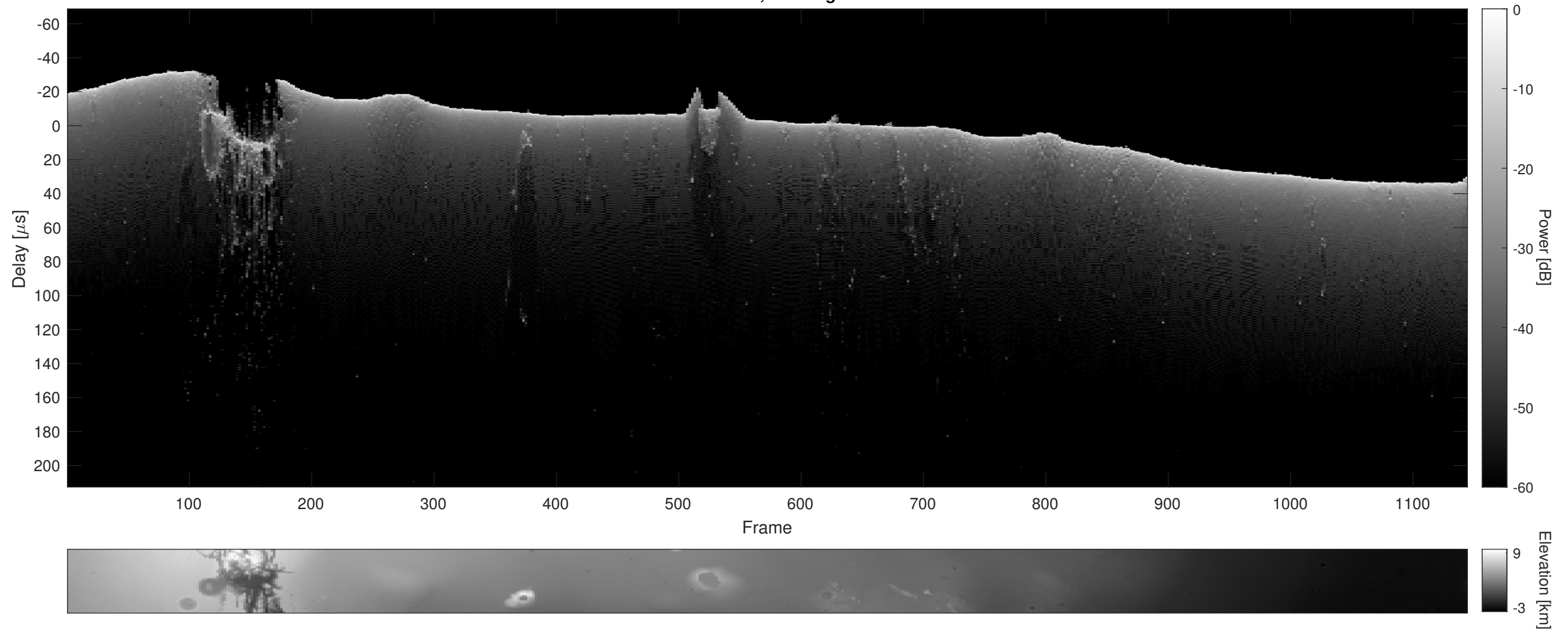
Orbit 10131, Cluttergram
