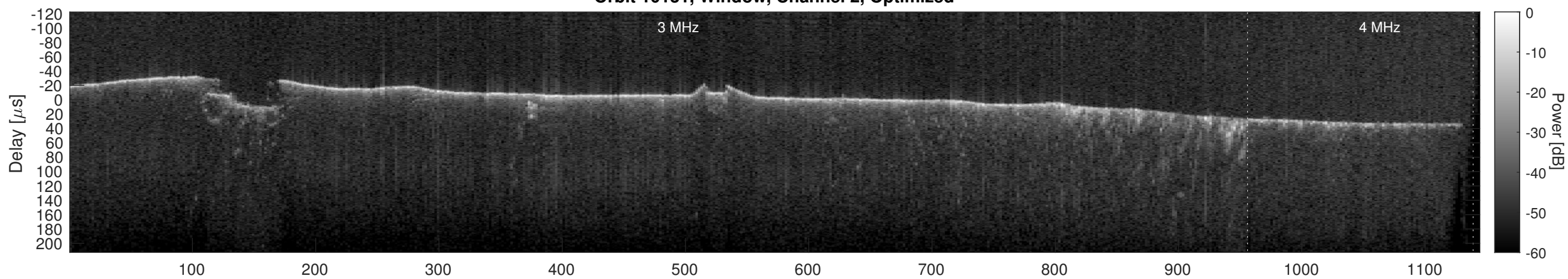
Orbit 10131, Cluttergram
