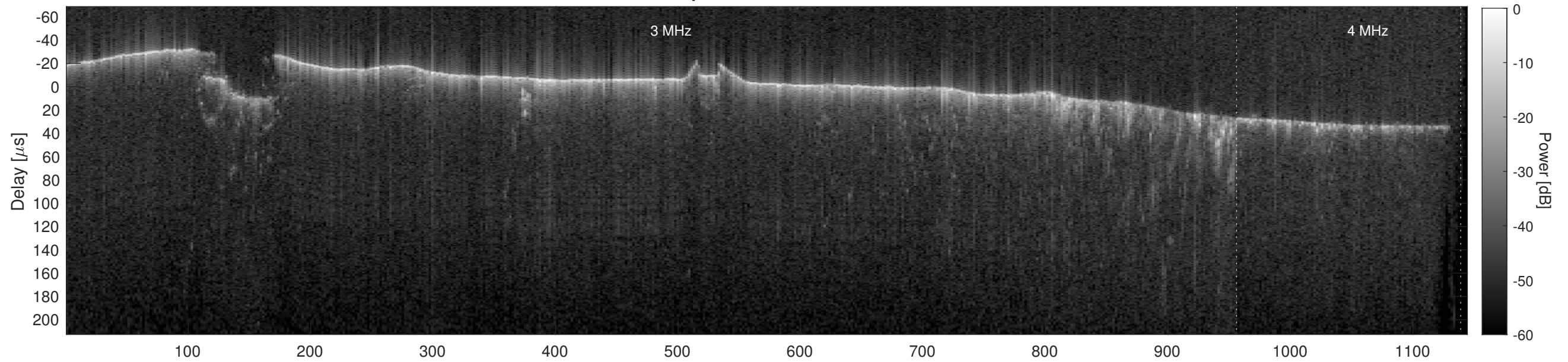
Orbit 10131, Cluttergram
