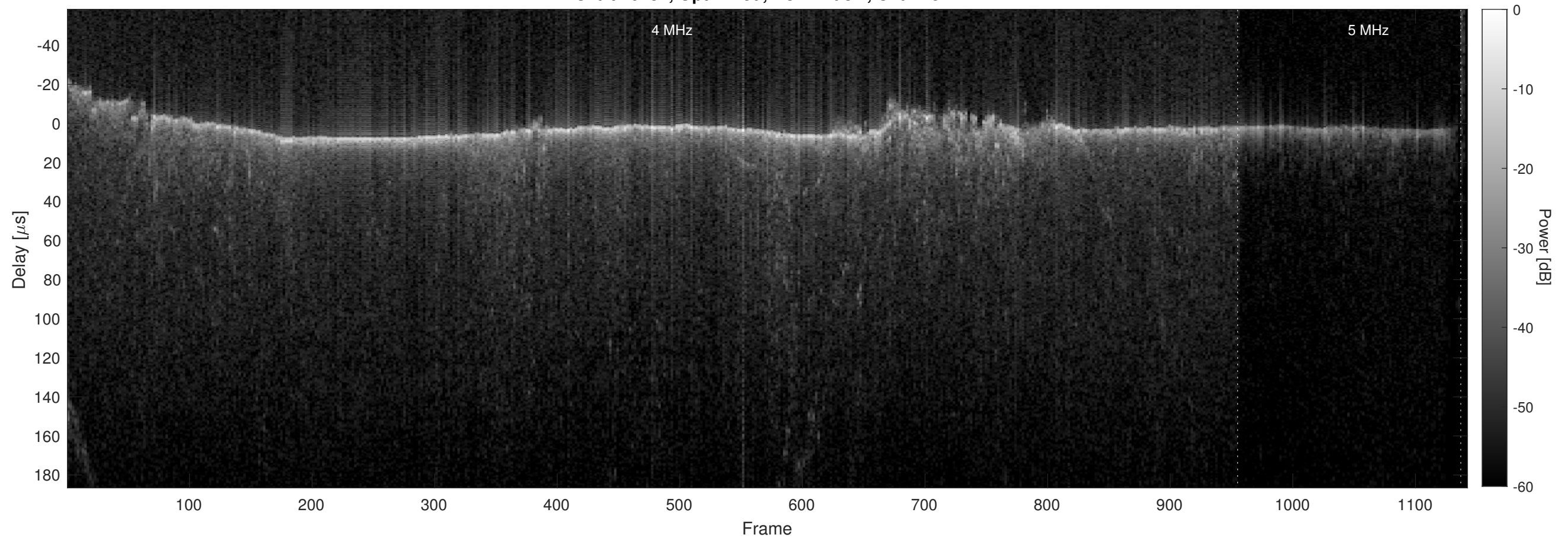
Orbit 10132, Optimized, No Window, Channel 2
