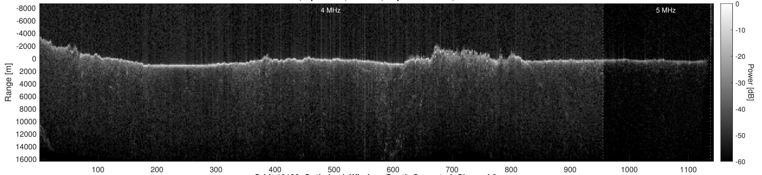
Orbit 10132, Optimized, Window, Depth-Corrected, Channel 2
