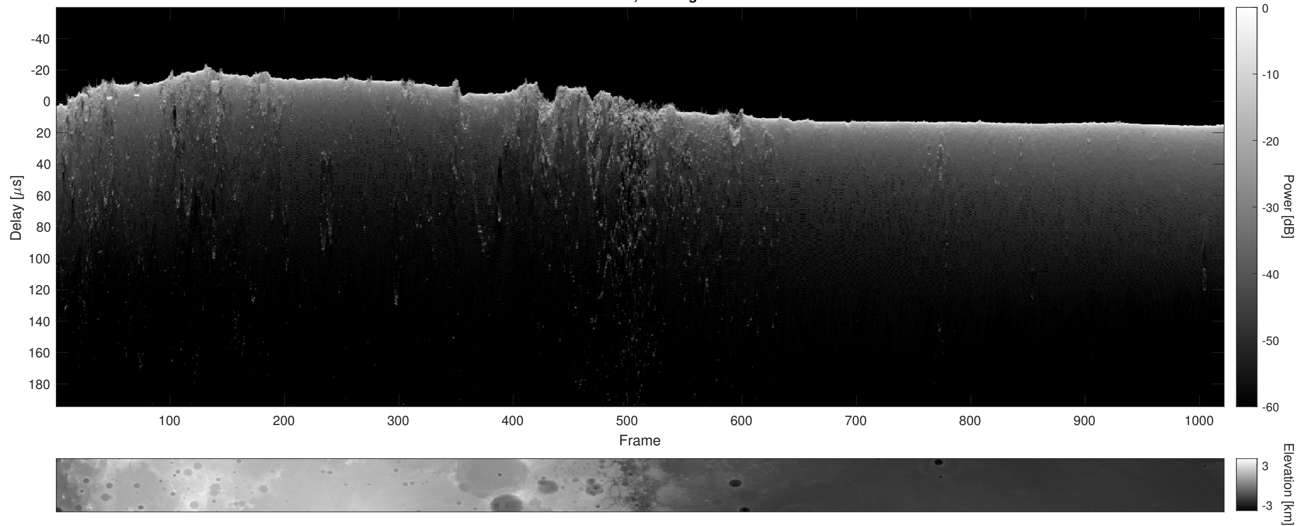
Orbit 10133, Cluttergram
