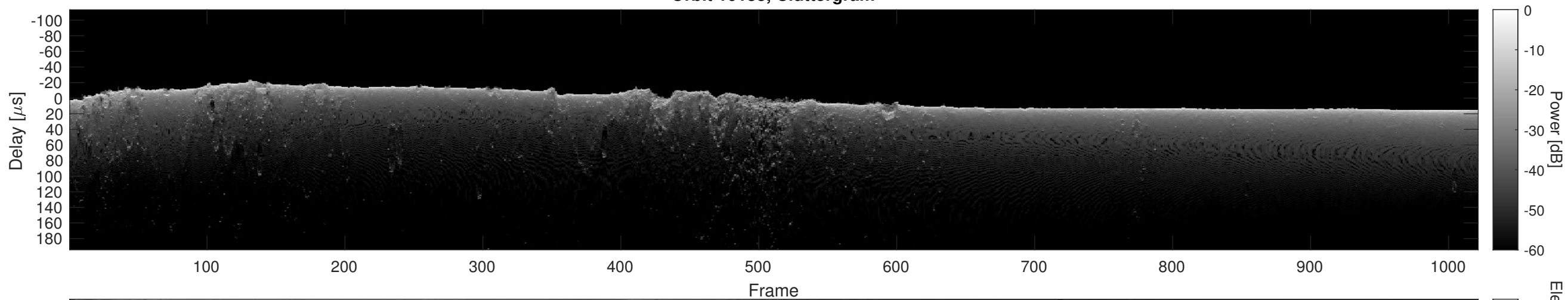
Orbit 10133, Cluttergram
