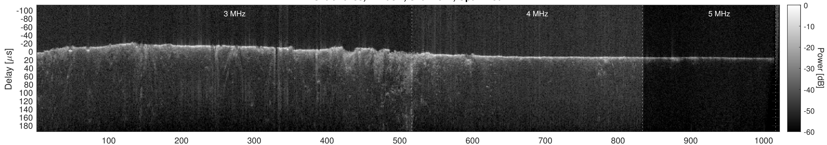
Orbit 10133, Cluttergram
