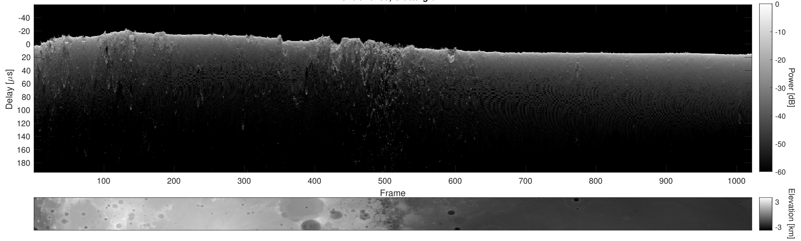
Orbit 10133, Cluttergram
