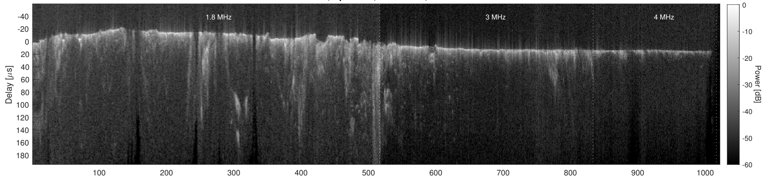
Orbit 10133, Cluttergram
