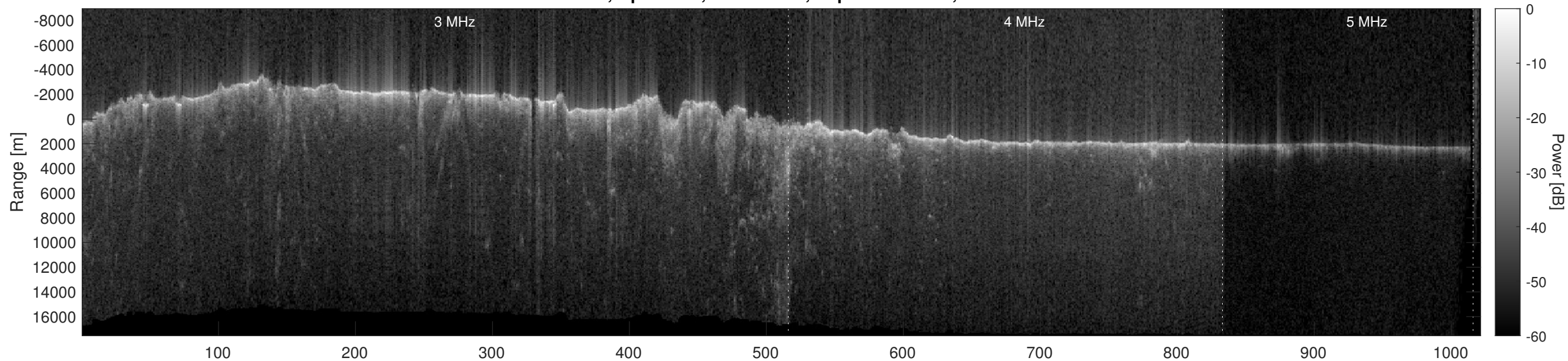
Orbit 10133, Optimized, No Window, Depth-Corrected, Channel 2
