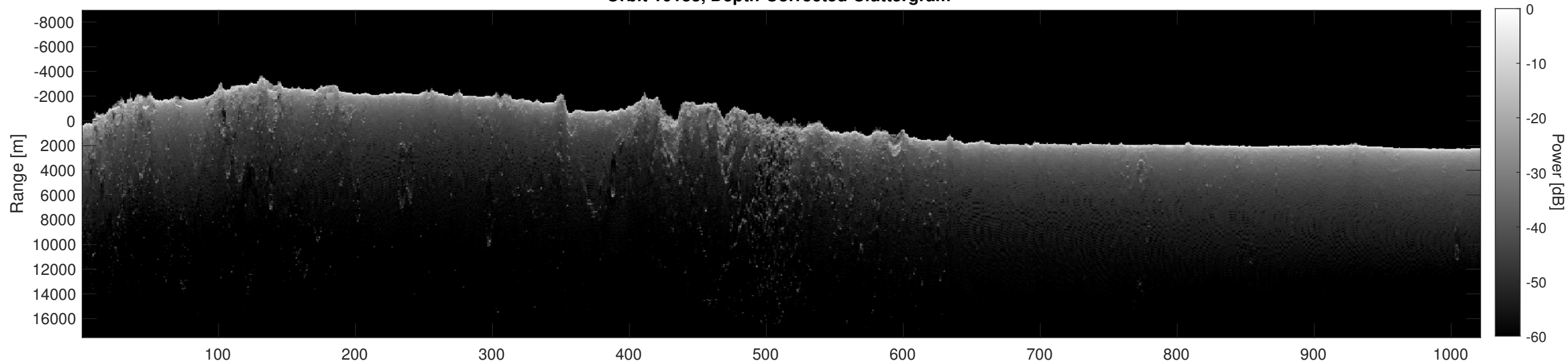
Orbit 10133, Depth-Corrected Cluttergram
