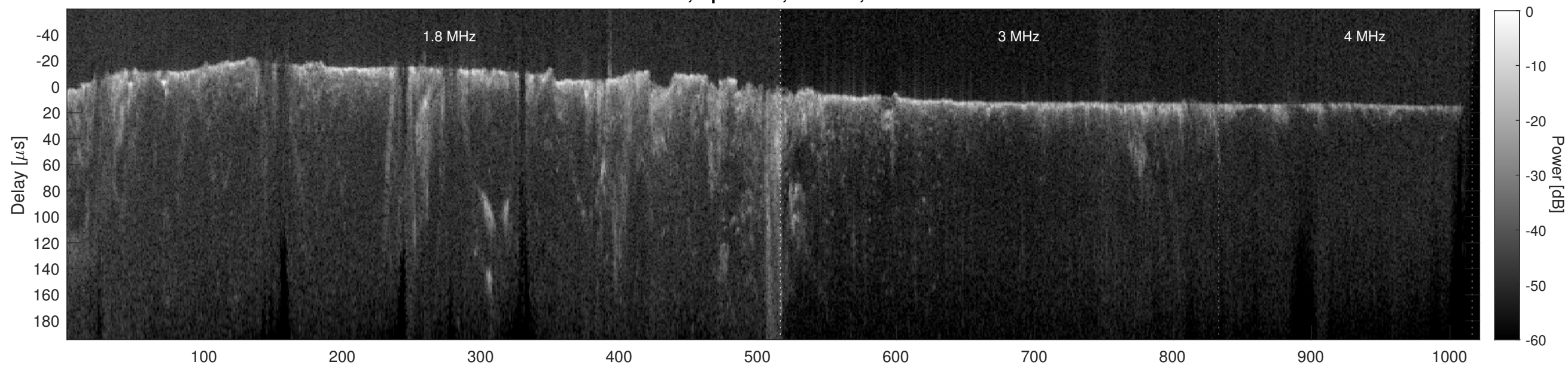
Orbit 10133, Cluttergram
