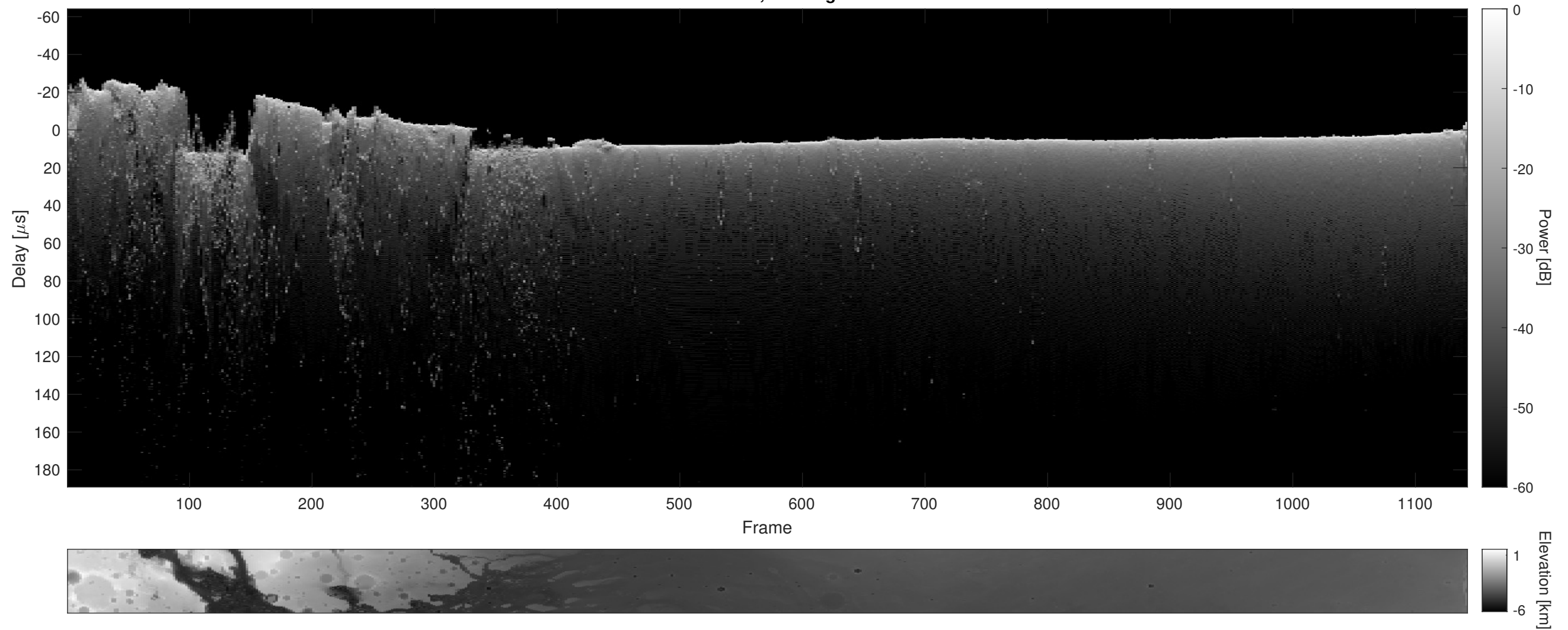
Orbit 10134, Cluttergram
