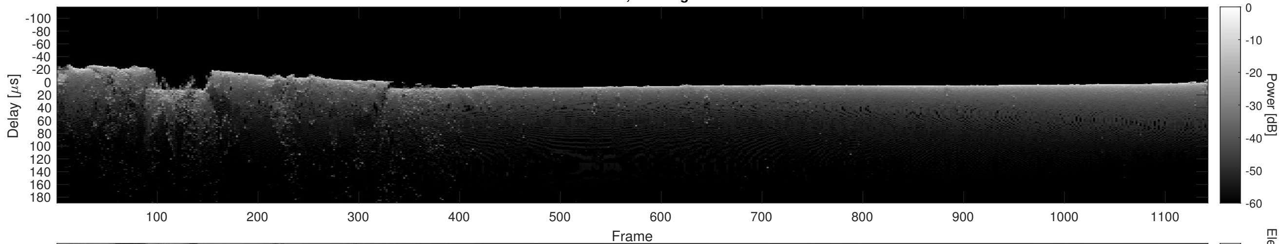
Orbit 10134, Cluttergram
