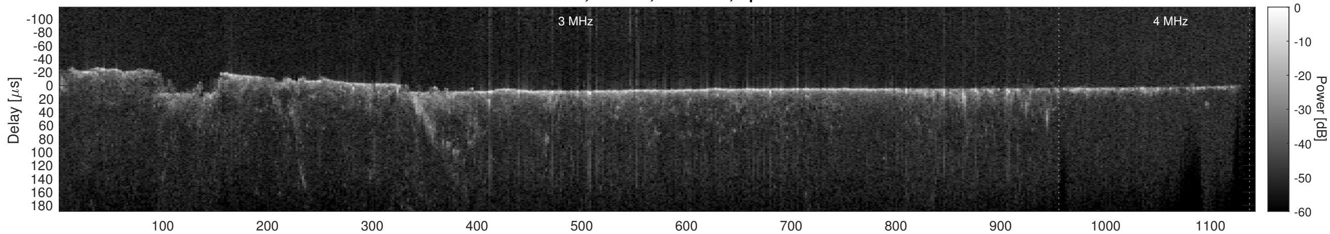
Orbit 10134, Cluttergram
